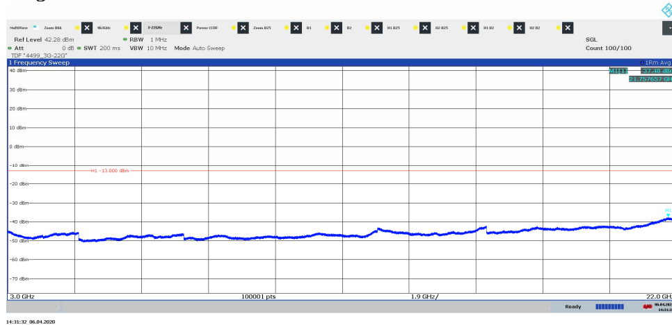
Diagram 3.4b, TM1, T, 3 GHz – 22 GHz, Port B:
