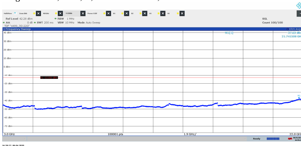
Diagram 3.11b, TM1, B, 3 GHz – 22 GHz, Port B:
