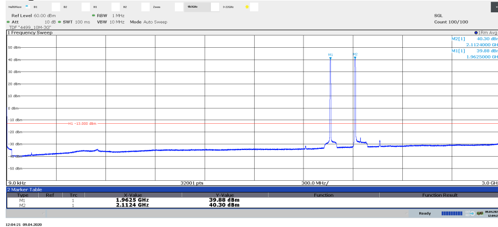
Diagram 3.13a, TM1, B, 9 kHz – 3 GHz, Port D:
