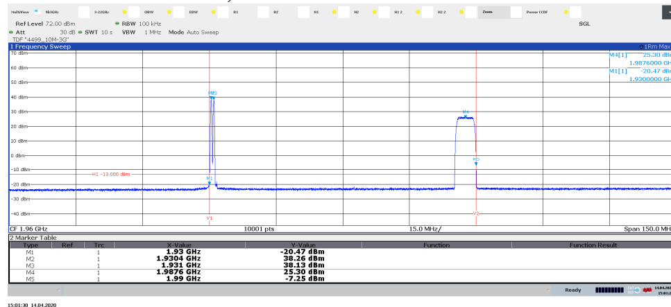
Diagram 3.23b, GSM: GMSK, NB IoT SA: N-TM, WCDMA: TM1, Bim G+IoT+W , 1.8875 GHz – 2.0375 GHz, Port A:
