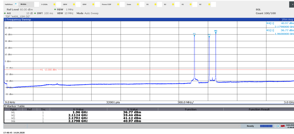
Diagram 3.22a, NB IoT SA: N-TM, WCDMA: TM1, \text{Tim}_{\text{IoT+W}} , 9 kHz – 3 GHz, Port B:
