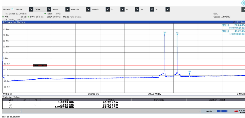
Diagram 3.3a, TM1, T, 9 kHz – 3 GHz, Port A:
