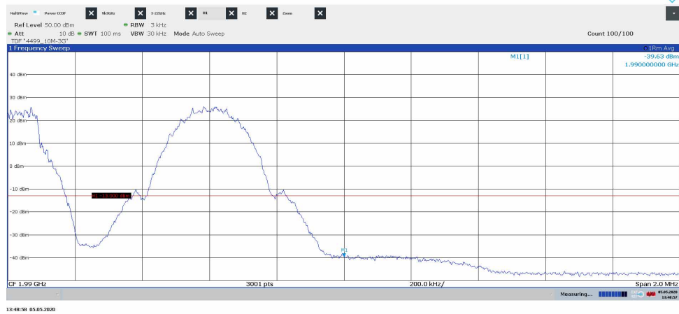
Diagram 2.38a, GSM: GMSK, NB IoT SA: N-TM, WCDMA: TM1, \text{Tim}_{G+IoT+W} , Port A:
