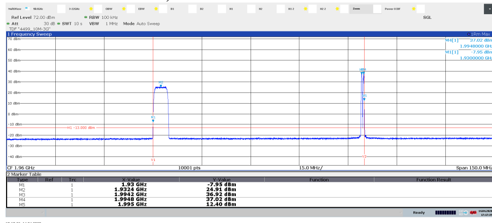
Diagram 3.20b, NB IoT SA: N-TM, WCDMA: TM1, \text{Tim}_{\text{IoT+W}} , 1.8875 GHz – 2.0375 GHz, Port A:
