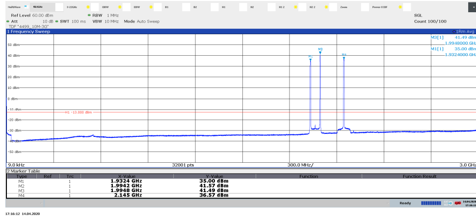
Diagram 3.20a, NB IoT SA: N-TM, WCDMA: TM1, \text{Tim}_{\text{IoT+W}} , 9 kHz – 3 GHz, Port A:
