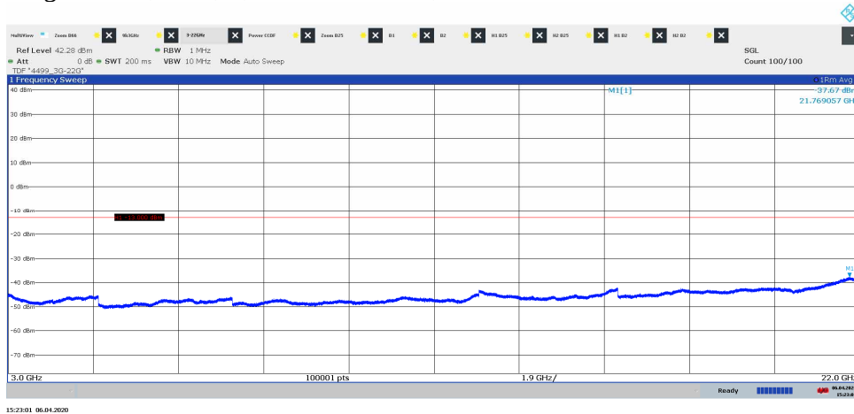
Diagram 3.5b, TM1, T, 3 GHz – 22 GHz, Port C:
