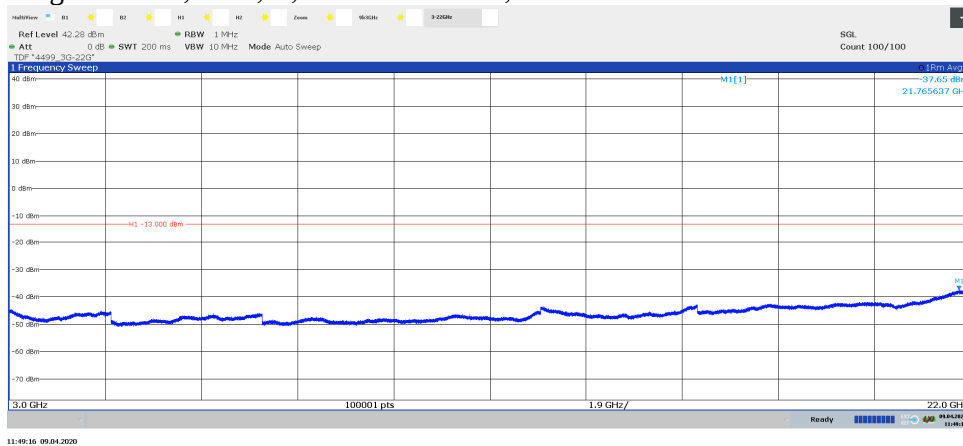
Diagram 3.12b, TM1, B, 3 GHz – 22 GHz, Port C:
