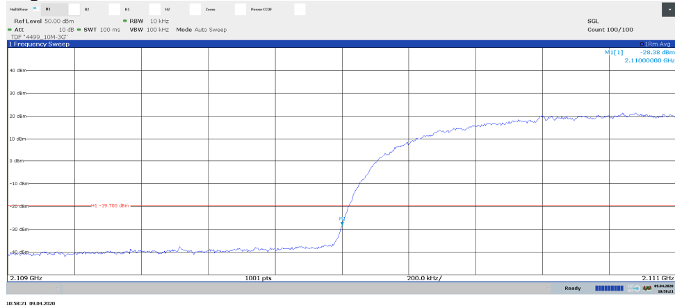
Diagram 2.20a, TM1, B, Port B:
