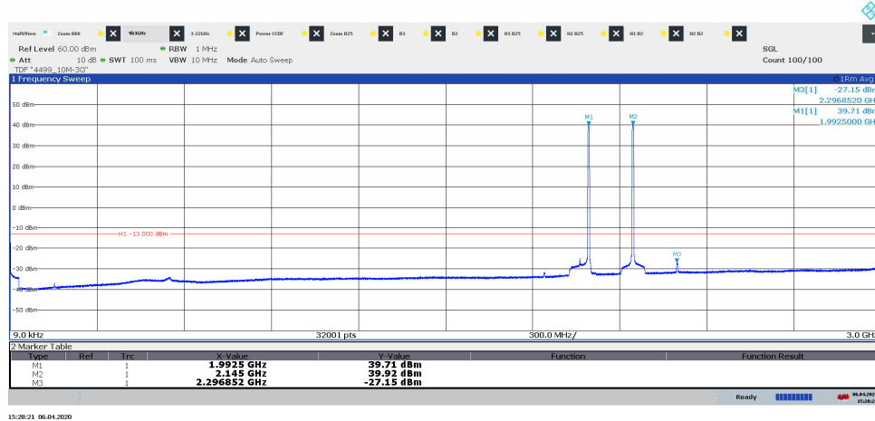
Diagram 3.6a, TM1, T, 9 kHz – 3 GHz, Port D:
