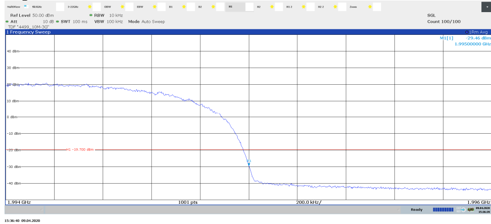
Diagram 2.8a, TM1, T, Port D:
