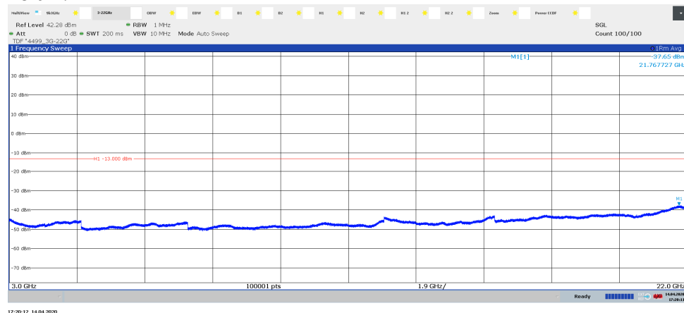
Diagram 3.20c, NB IoT SA: N-TM, WCDMA: TM1, \text{Tim}_{\text{IoT+W}} , 3 GHz – 22 GHz, Port A:
