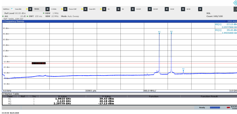
Diagram 3.5a, TM1, T, 9 kHz – 3 GHz, Port C:
