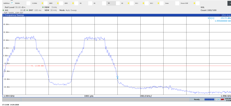
Diagram 2.34a, NB IoT SA: N-TM, WCDMA: TM1, \text{Tim}_{\text{IoT+W}} , Port A:
