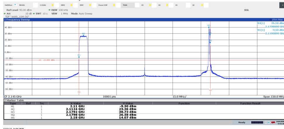
Diagram 3.22b, NB IoT SA: N-TM, WCDMA: TM1, \text{Tim}_{\text{IoT+W}} , 2.07 GHz – 2.22 GHz, Port B:
