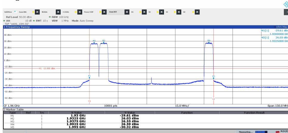
Diagram 3.7b, TM1, Bim, 1.8875 GHz – 2.0375 GHz, Port A:
