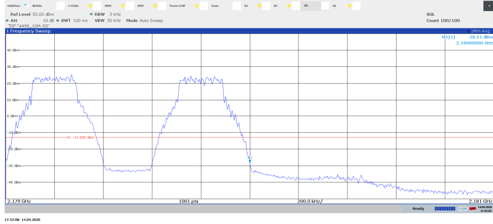
Diagram 2.36a, NB IoT SA: N-TM, WCDMA: TM1, \text{Tim}_{\text{IoT+W}} , Port B:
