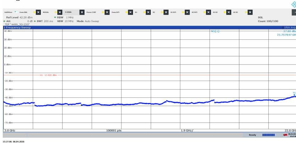
Diagram 3.6b, TM1, T, 3 GHz – 22 GHz, Port D:
