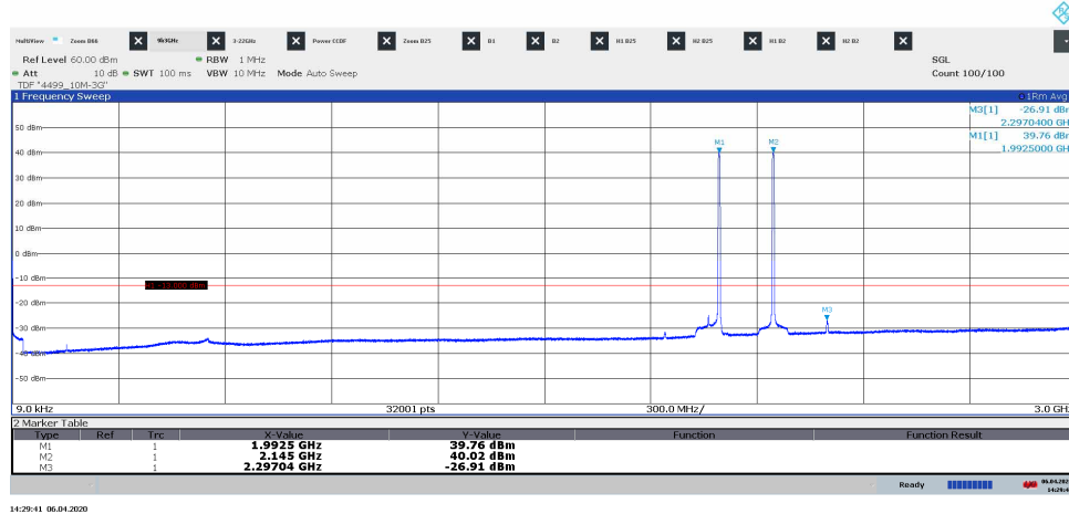
Diagram 3.4a, TM1, T, 9 kHz – 3 GHz, Port B:
