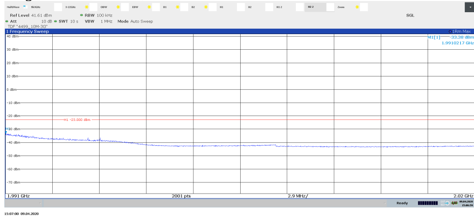
Diagram 2.16b, TM1, T, Port B:
