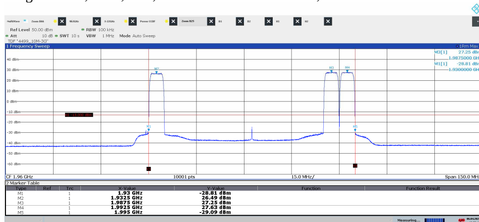
Diagram 3.8b, TM1, Tim, 1.8875 GHz – 2.0375 GHz, Port A:
