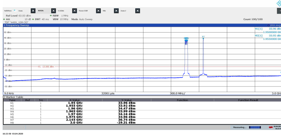
Diagram 3.9a, TM1, M6, 9 kHz – 3 GHz, Port A:
