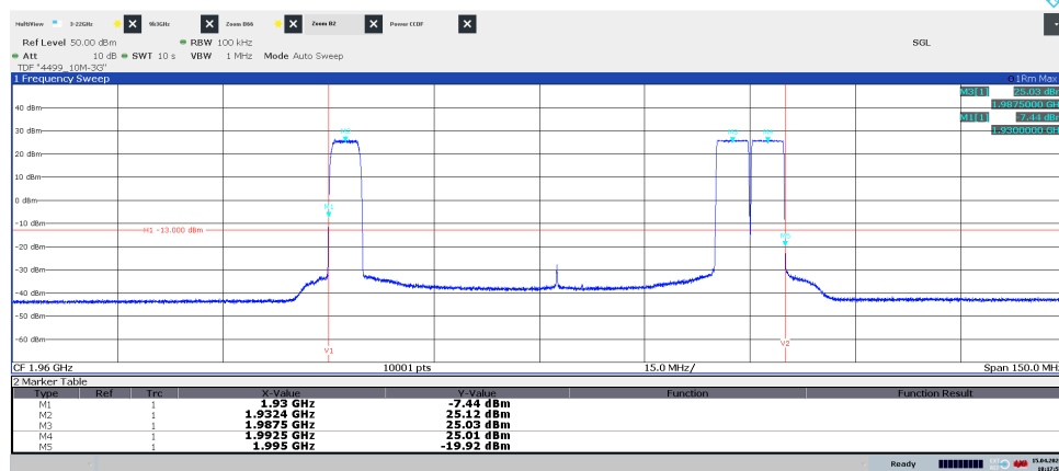
Diagram 3.2b, WCDMA TM1, LTE: E-TM1.1, \text{Tim}_{W+L} , 1.8875 GHz – 2.0375 GHz, Port A:
