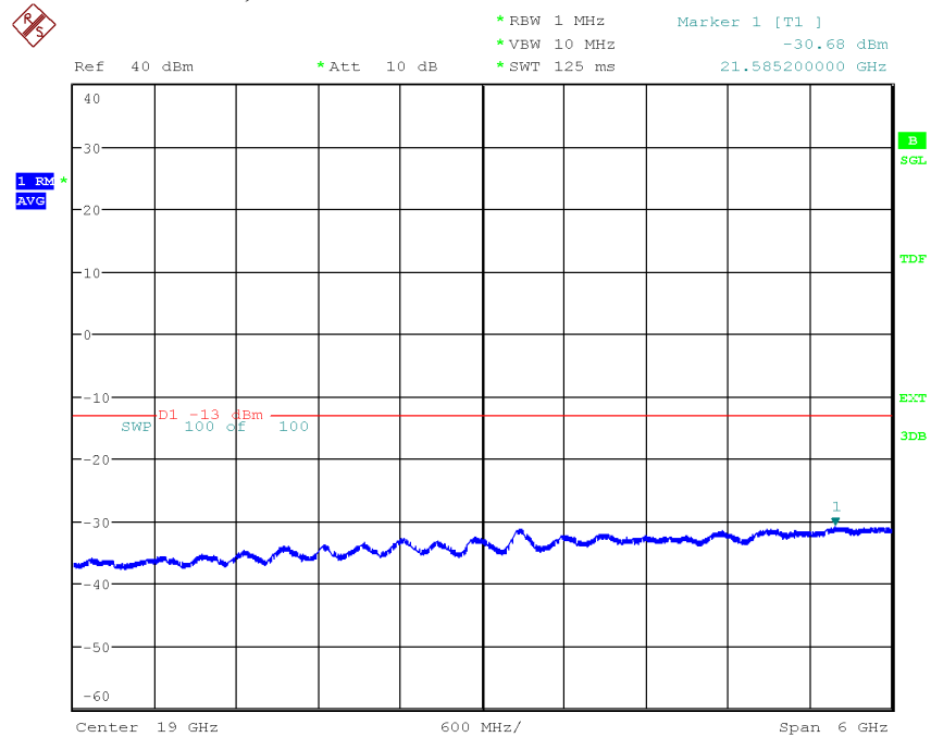
Diagram 3.6e, WCDMA: TM1, LTE: E-TM1.1, BMT6, 16 GHz – 22 GHz, Port B:
