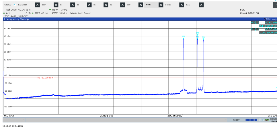
Diagram 3.9a, WCDMA: TM1, LTE: E-TM1.1, Bim W+L+IoT , 9 kHz – 3 GHz, Port B:
