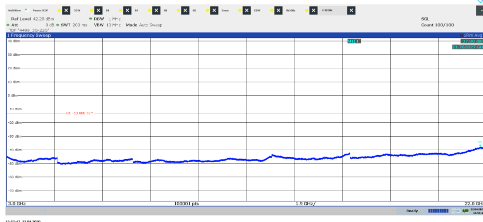
Diagram 3.8c, WCDMA: TM1, LTE: E-TM1.1, \text{Tim}_{W+L+IoT} , 3 GHz – 22 GHz, Port A:
