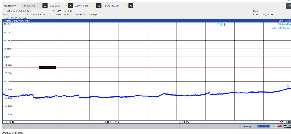
Diagram 3.5c, WCDMA TM1, LTE: E-TM1.1, \text{Tim}_{W+L} , 3 GHz – 22 GHz, Port B:
