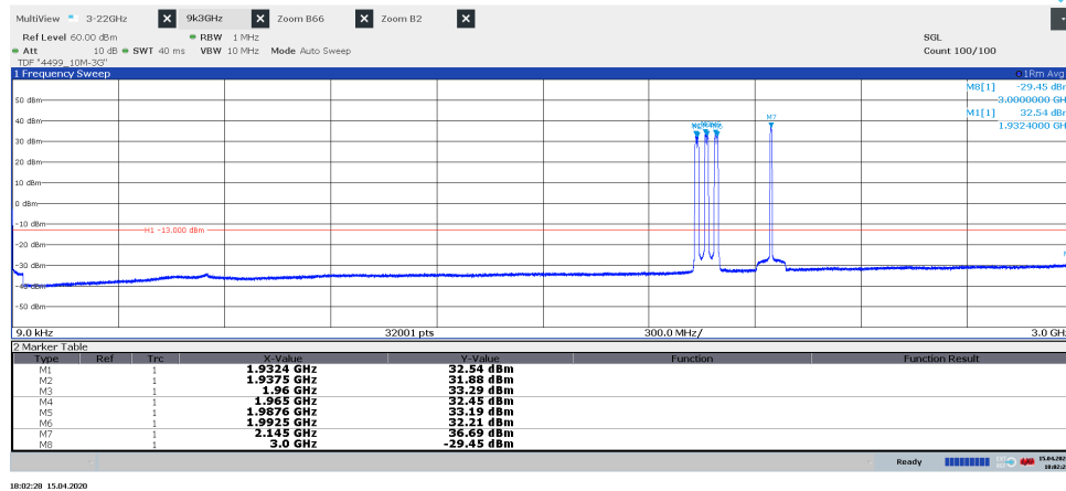
Diagram 3.3a, WCDMA TM1, LTE: E-TM1.1, BMT6, 9 kHz – 3 GHz, Port A:
