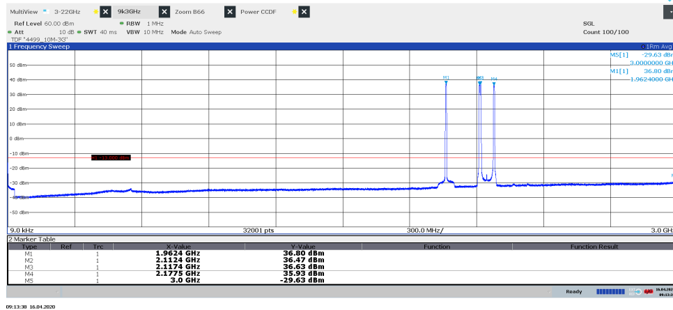
Diagram 3.4a, WCDMA TM1, LTE: E-TM 1.1, Bim W+L , 9 kHz – 3 GHz, Port B:
