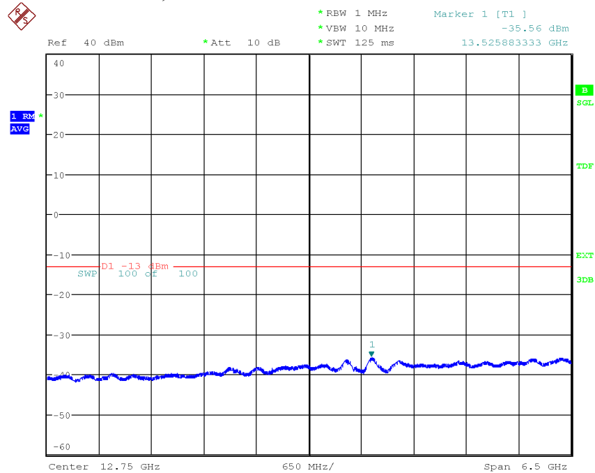
Diagram 3.6d, WCDMA: TM1, LTE: E-TM1.1, BMT6, 9.5 GHz – 16 GHz, Port B:
