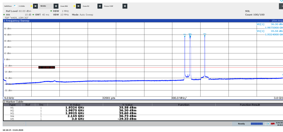
Diagram 3.2a, WCDMA TM1, LTE: E-TM1.1, \text{Tim}_{W+L} , 9 kHz – 3 GHz, Port A:
