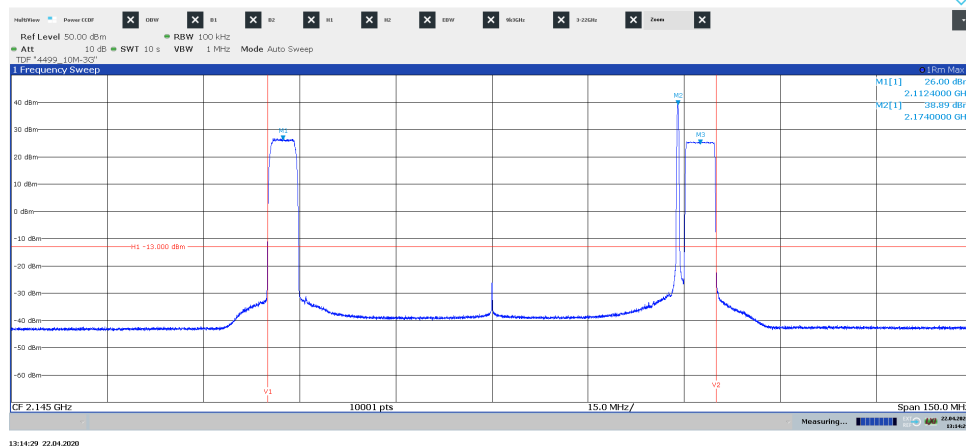
Diagram 3.10b, WCDMA: TM1, LTE: E-TM1.1, \text{Tim}_{\text{W}+\text{L}+\text{IoT}} , 2.070 GHz – 2.220 GHz, Port B:
