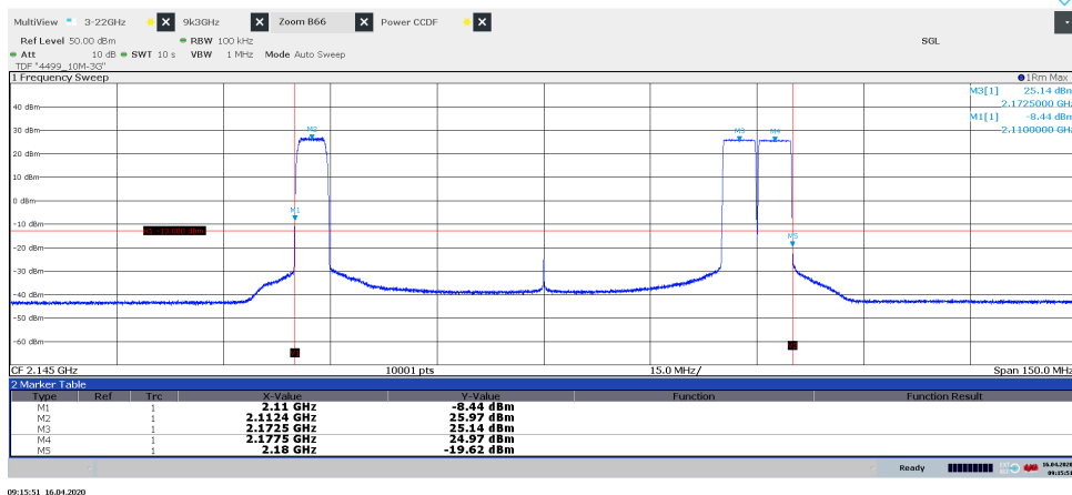
Diagram 3.5b, WCDMA TM1, LTE: E-TM1.1, \text{Tim}_{W+L} , 2.070 GHz – 2.220 GHz, Port B:
