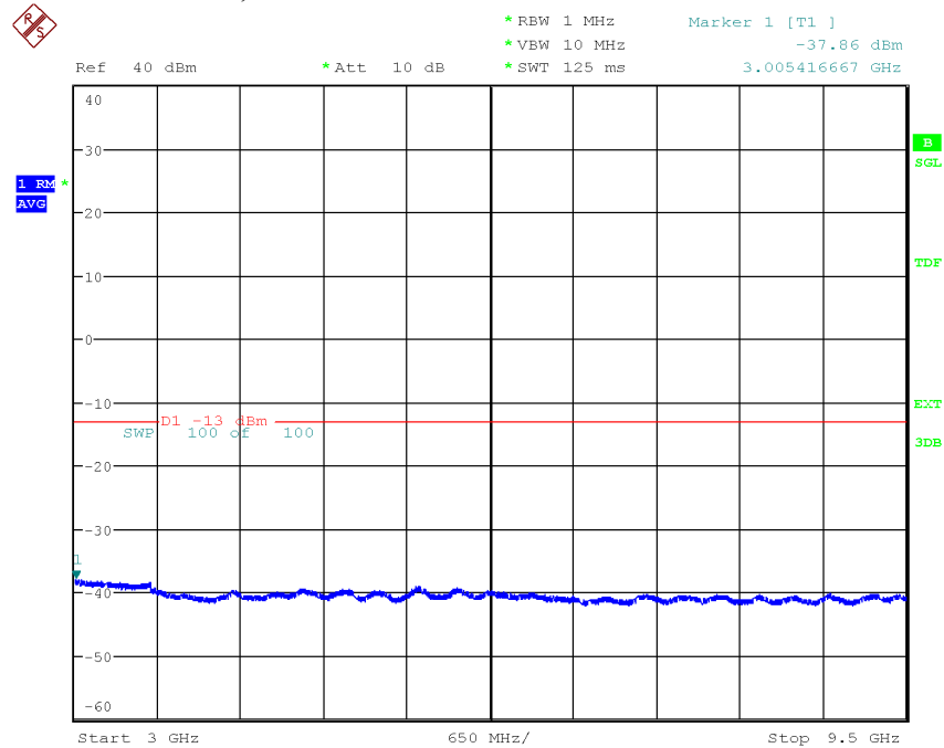
Diagram 3.6c, WCDMA: TM1, LTE: E-TM1.1, BMT6, 3 GHz – 9.5 GHz, Port B:
