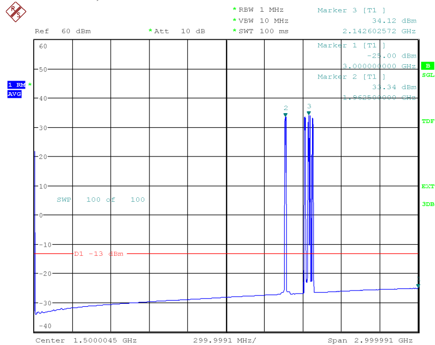
Diagram 3.6a, WCDMA: TM1, LTE: E-TM1.1, BMT6, 9 kHz – 3 GHz, Port B:
