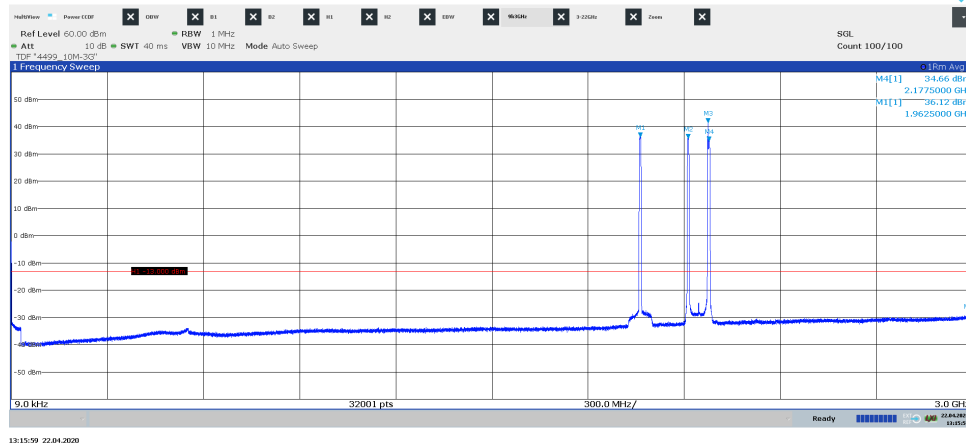
Diagram 3.10a, WCDMA: TM1, LTE: E-TM1.1, \text{Tim}_{\text{W}+\text{L}+\text{IoT}} , 9 kHz – 3 GHz, Port B:
