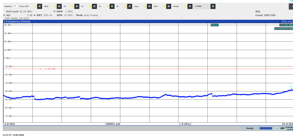
Diagram 3.10c, WCDMA: TM1, LTE: E-TM1.1, \text{Tim}_{\text{W}+\text{L}+\text{IoT}} , 3 GHz – 22 GHz, Port B:
