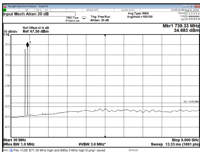
Figure 8.2-203: Conducted spurious emissions at Port C, QPSK, multi-band Band 71 20 MHz high channel and Band 85A 5 MHz high channel
