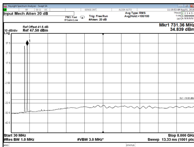
Figure 8.2-172: Conducted spurious emissions at Port D, QPSK, multi-band Band 71 10 MHz low channel and Band 85A 10 MHz low channel
