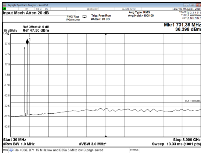
Figure 8.2-183: Conducted spurious emissions at Port C, QPSK, multi-band Band 71 15 MHz low channel and Band 85A 5 MHz low channel
