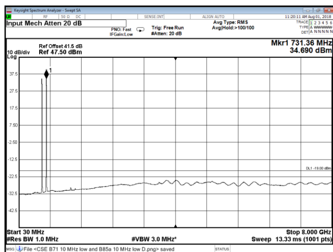
Figure 8.2-171: Conducted spurious emissions at Port C, QPSK, multi-band Band 71 10 MHz low channel and Band 85A 10 MHz low channel
