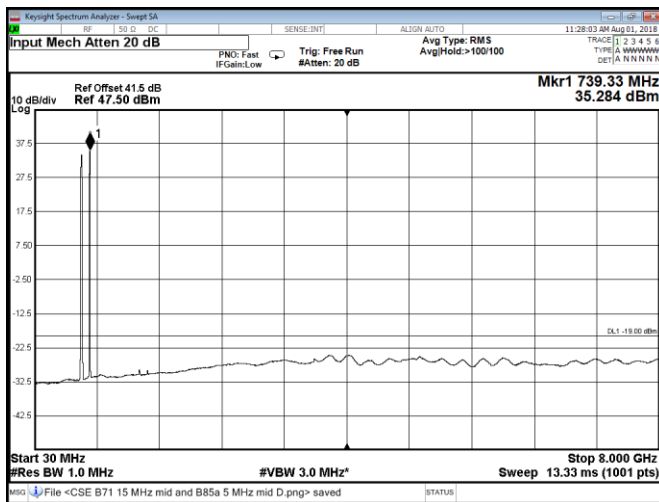
Figure 8.2-187: Conducted spurious emissions at Port C, QPSK, multi-band Band 71 15 MHz mid channel and Band 85A 5 MHz mid channel
