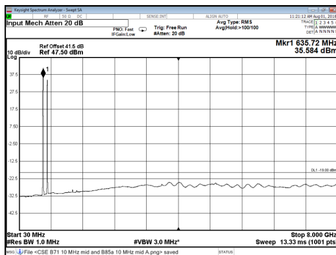
Figure 8.2-174: Conducted spurious emissions at Port B, QPSK, multi-band Band 71 10 MHz mid channel and Band 85A 10 MHz mid channel
