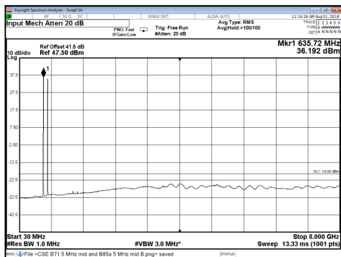
Figure 8.2-161: Conducted spurious emissions at Port A, QPSK, multi-band Band 71 5 MHz mid channel and Band 85A 5 MHz mid channel
