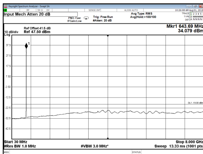
Figure 8.2-96: Conducted spurious emissions at Port D, QPSK, Band 71 high 15 MHz channel + IoT carrier
