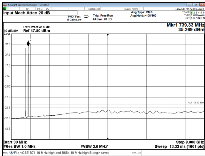
Figure 8.2-177: Conducted spurious emissions at Port A, QPSK, multi-band Band 71 10 MHz high channel and Band 85A 10 MHz high channel
