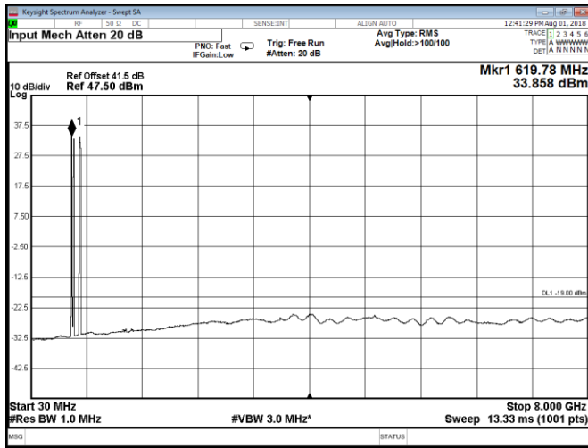
Figure 8.2-205: Conducted spurious emissions at Port A, QPSK, multi-band Band 71 two 5 MHz channels and Band 85A two 5 MHz channels
