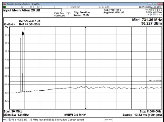
Figure 8.2-184: Conducted spurious emissions at Port D, QPSK, multi-band Band 71 15 MHz low channel and Band 85A 5 MHz low channel
