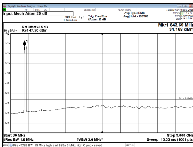
Figure 8.2-192: Conducted spurious emissions at Port D, QPSK, multi-band Band 71 15 MHz high channel and Band 85A 5 MHz high channel
