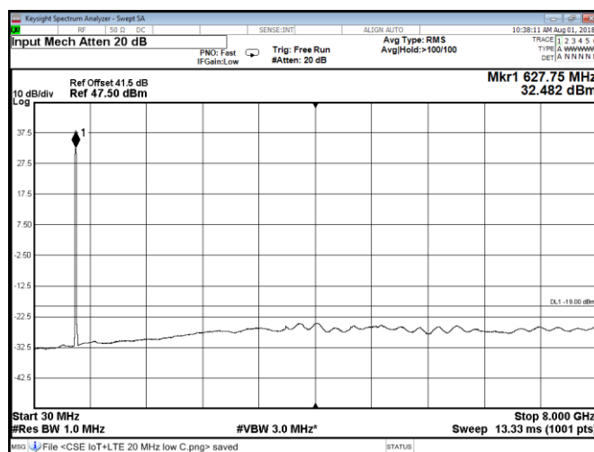
Figure 8.2-100: Conducted spurious emissions at Port D, QPSK, Band 71 low 20 MHz channel + IoT carrier
