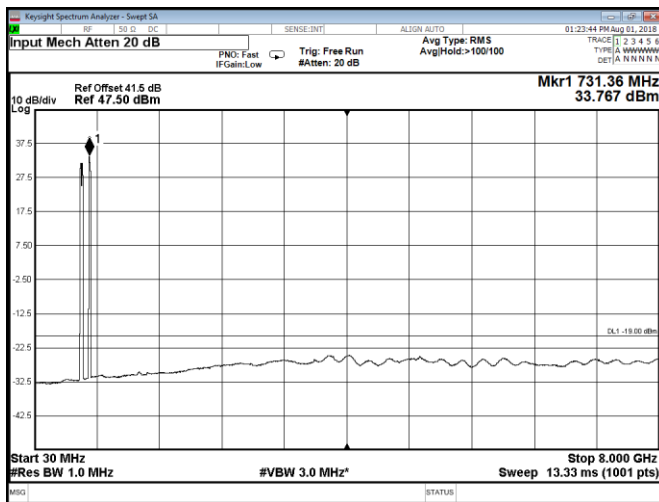
Figure 8.2-215: Conducted spurious emissions at Port C, QPSK, multi-band Band 71 two 15 MHz channels and Band 85A three 5 MHz channels
