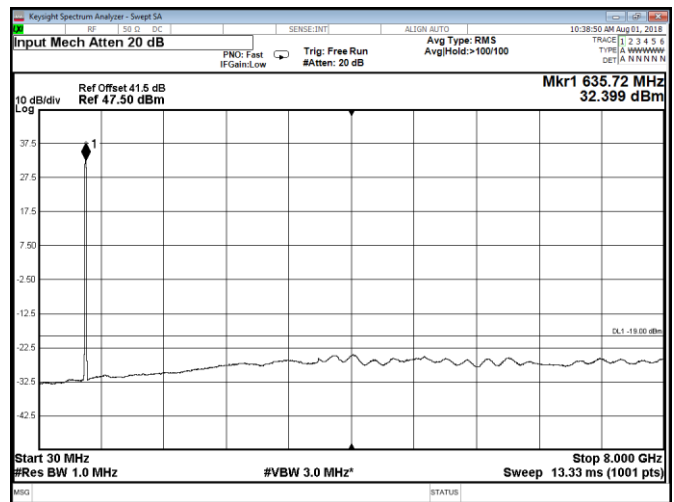
Figure 8.2-104: Conducted spurious emissions at Port D, QPSK, Band 71 mid 20 MHz channel + IoT carrier
