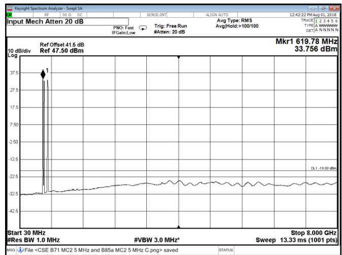
Figure 8.2-208: Conducted spurious emissions at Port D, QPSK, multi-band Band 71 two 5 MHz channels and Band 85A two 5 MHz channels
