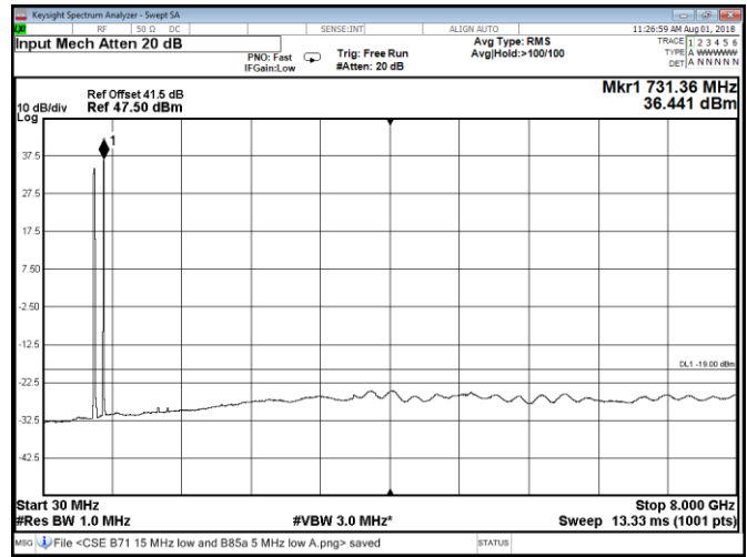
Figure 8.2-182: Conducted spurious emissions at Port B, QPSK, multi-band Band 71 15 MHz low channel and Band 85A 5 MHz low channel
