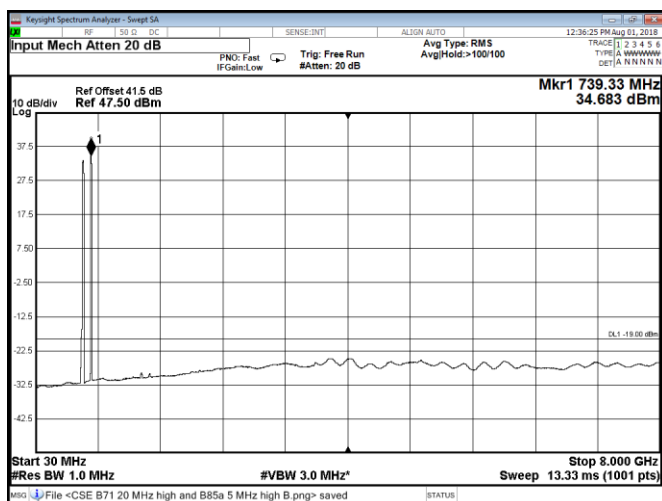
Figure 8.2-201: Conducted spurious emissions at Port A, QPSK, multi-band Band 71 20 MHz high channel and Band 85A 5 MHz high channel
