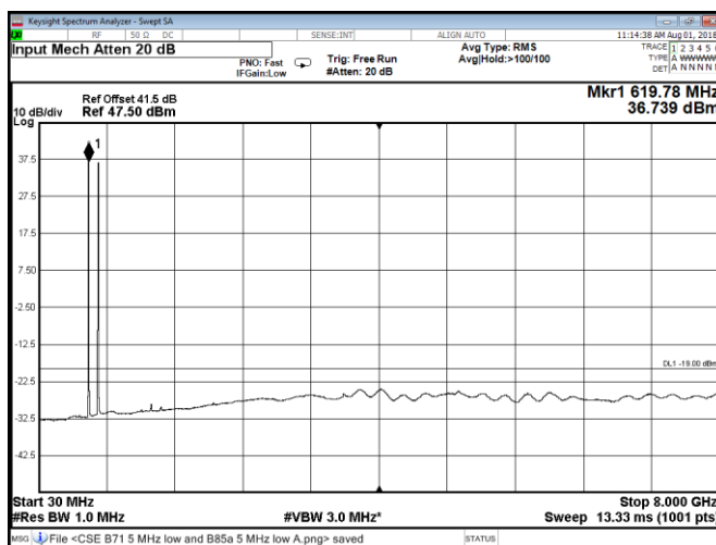
Figure 8.2-158: Conducted spurious emissions at Port B, QPSK, multi-band Band 71 5 MHz low channel and Band 85A 5 MHz low channel
