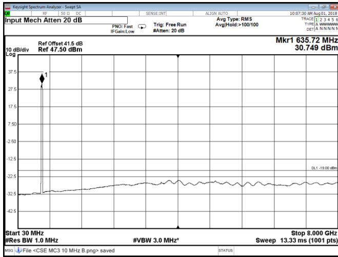
Figure 8.2-145: Conducted spurious emissions at Port A, QPSK, Band 71 multi carrier three 10 MHz channels
