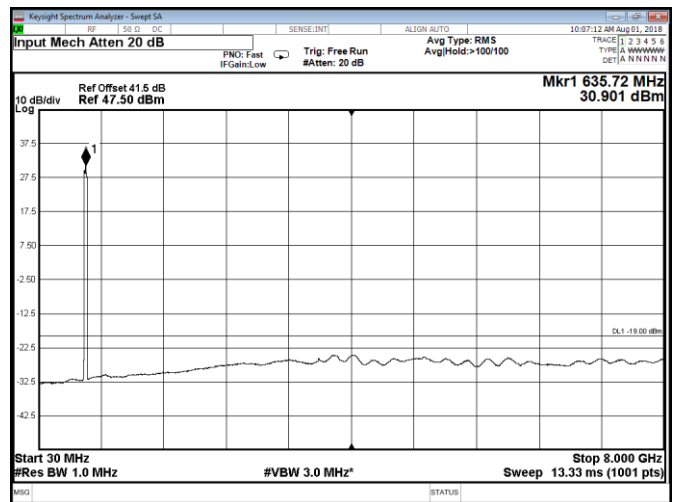
Figure 8.2-148: Conducted spurious emissions at Port D, QPSK, Band 71 multi carrier three 10 MHz channels
