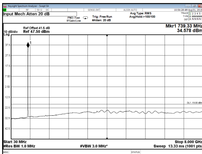
Figure 8.2-114: Conducted spurious emissions at Port B, QPSK, Band 85A mid 10 MHz channel + IoT carrier
