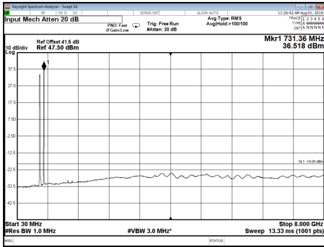
Figure 8.2-181: Conducted spurious emissions at Port A, QPSK, multi-band Band 71 15 MHz low channel and Band 85A 5 MHz low channel
