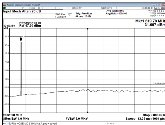
Figure 8.2-134: Conducted spurious emissions at Port B, QPSK, Band 71 multi carrier two 10 MHz channels
