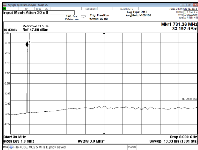
Figure 8.2-151: Conducted spurious emissions at Port C, QPSK, Band 85A multi carrier two 5 MHz channels
