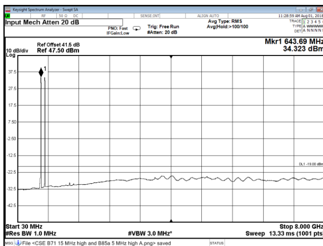
Figure 8.2-190: Conducted spurious emissions at Port B, QPSK, multi-band Band 71 15 MHz high channel and Band 85A 5 MHz high channel
