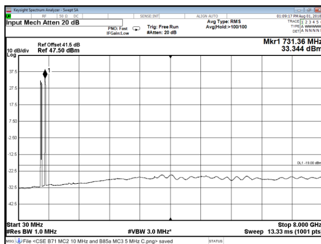
Figure 8.2-212: Conducted spurious emissions at Port D, QPSK, multi-band Band 71 two 10 MHz channels and Band 85A three 5 MHz channels
