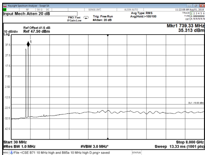
Figure 8.2-179: Conducted spurious emissions at Port C, QPSK, multi-band Band 71 10 MHz high channel and Band 85A 10 MHz high channel
