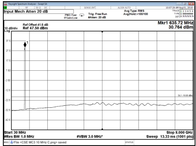
Figure 8.2-146: Conducted spurious emissions at Port B, QPSK, Band 71 multi carrier three 10 MHz channels
