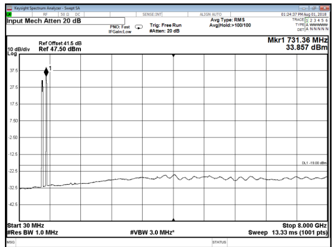
Figure 8.2-216: Conducted spurious emissions at Port D, QPSK, multi-band Band 71 two 15 MHz channels and Band 85A three 5 MHz channels
