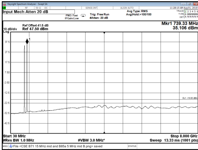
Figure 8.2-185: Conducted spurious emissions at Port A, QPSK, multi-band Band 71 15 MHz mid channel and Band 85A 5 MHz mid channel
