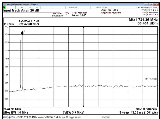
Figure 8.2-196: Conducted spurious emissions at Port D, QPSK, multi-band Band 71 20 MHz low channel and Band 85A 5 MHz low channel
