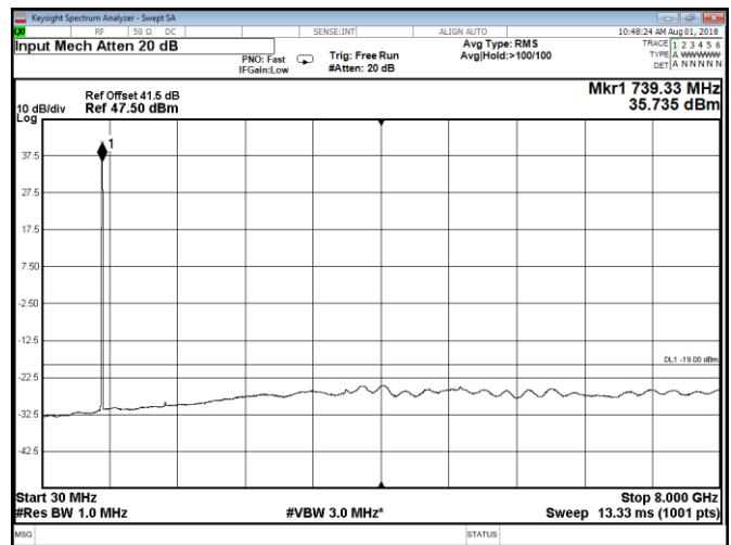
Figure 8.2-120: Conducted spurious emissions at Port D, QPSK, Band 85A high 10 MHz channel + IoT carrier
