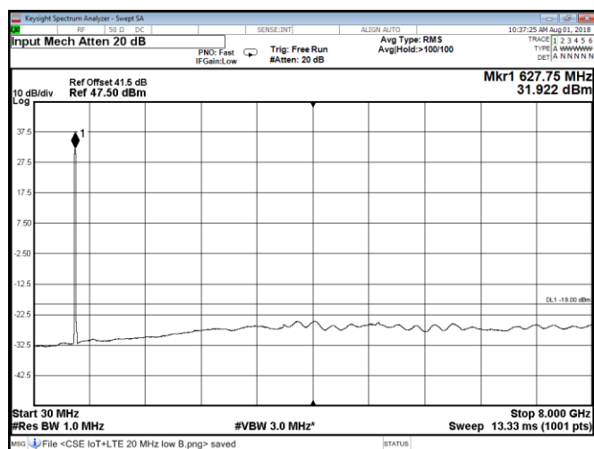
Figure 8.2-99: Conducted spurious emissions at Port C, QPSK, Band 71 low 20 MHz channel + IoT carrier
