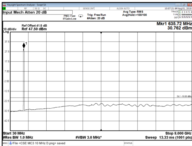
Figure 8.2-147: Conducted spurious emissions at Port C, QPSK, Band 71 multi carrier three 10 MHz channels
