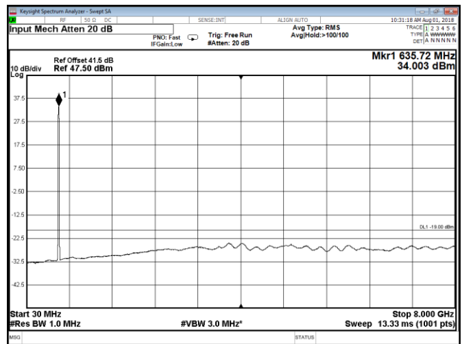
Figure 8.2-92: Conducted spurious emissions at Port D, QPSK, Band 71 mid 15 MHz channel + IoT carrier
