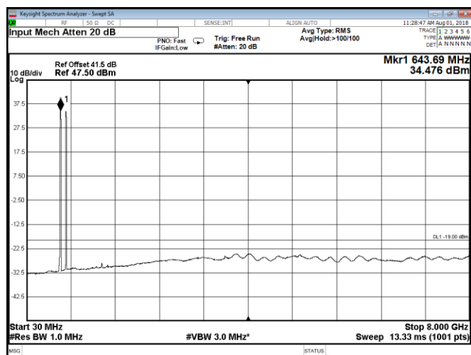
Figure 8.2-189: Conducted spurious emissions at Port A, QPSK, multi-band Band 71 15 MHz high channel and Band 85A 5 MHz high channel
