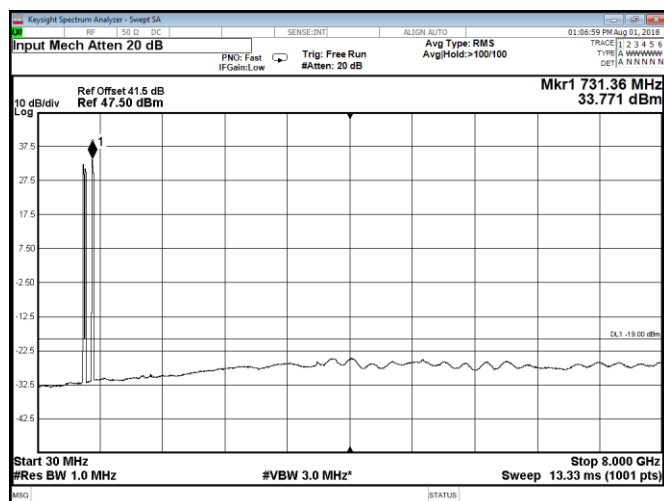
Figure 8.2-209: Conducted spurious emissions at Port A, QPSK, multi-band Band 71 two 10 MHz channels and Band 85A three 5 MHz channels
