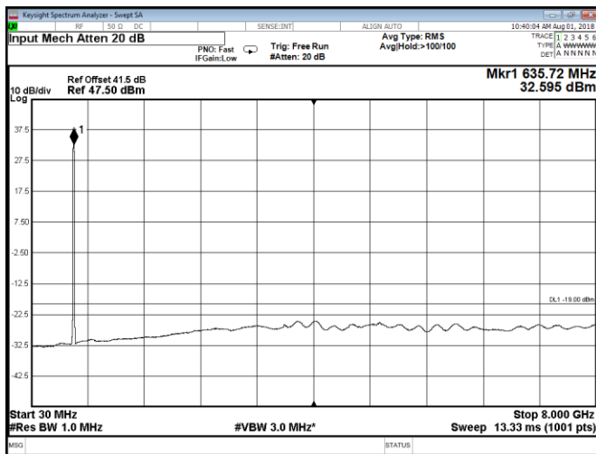
Figure 8.2-103: Conducted spurious emissions at Port C, QPSK, Band 71 mid 20 MHz channel + IoT carrier
