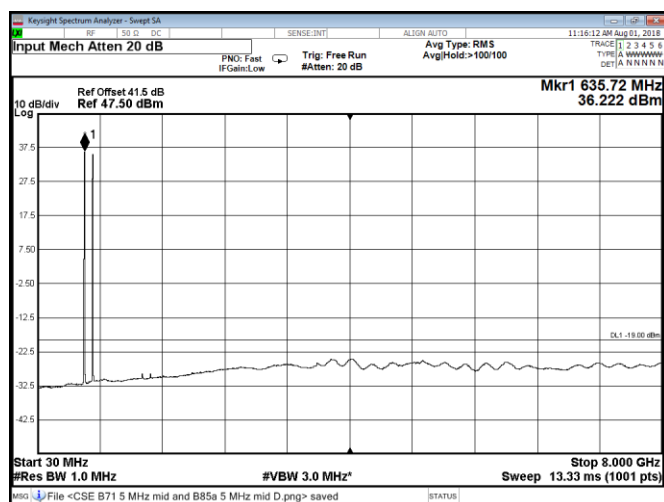
Figure 8.2-163: Conducted spurious emissions at Port C, QPSK, multi-band Band 71 5 MHz mid channel and Band 85A 5 MHz mid channel
