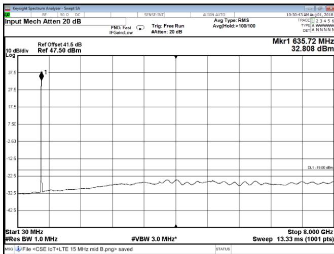
Figure 8.2-91: Conducted spurious emissions at Port C, QPSK, Band 71 mid 15 MHz channel + IoT carrier
