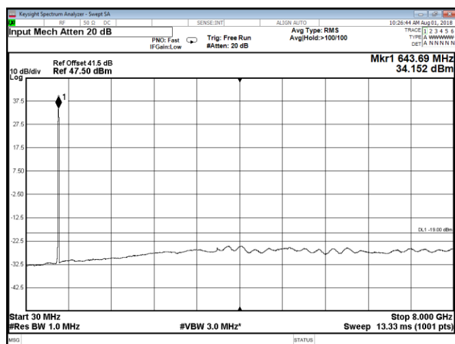
Figure 8.2-95: Conducted spurious emissions at Port C, QPSK, Band 71 high 15 MHz channel + IoT carrier
