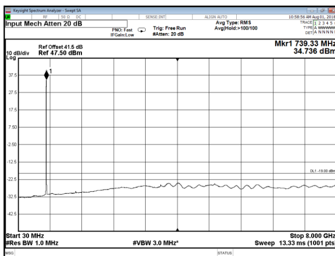
Figure 8.2-116: Conducted spurious emissions at Port D, QPSK, Band 85A mid 10 MHz channel + IoT carrier
