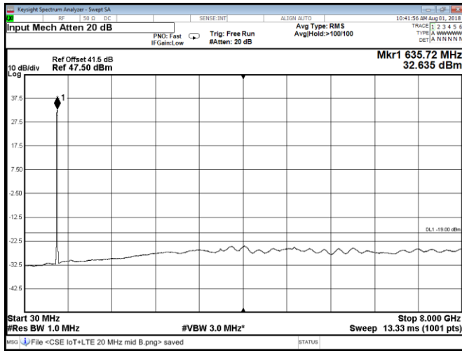
Figure 8.2-101: Conducted spurious emissions at Port A, QPSK, Band 71 mid 20 MHz channel + IoT carrier
