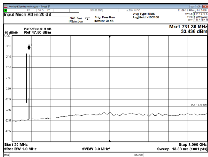
Figure 8.2-211: Conducted spurious emissions at Port C, QPSK, multi-band Band 71 two 10 MHz channels and Band 85A three 5 MHz channels
