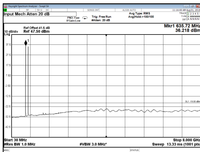
Figure 8.2-164: Conducted spurious emissions at Port D, QPSK, multi-band Band 71 5 MHz mid channel and Band 85A 5 MHz mid channel
