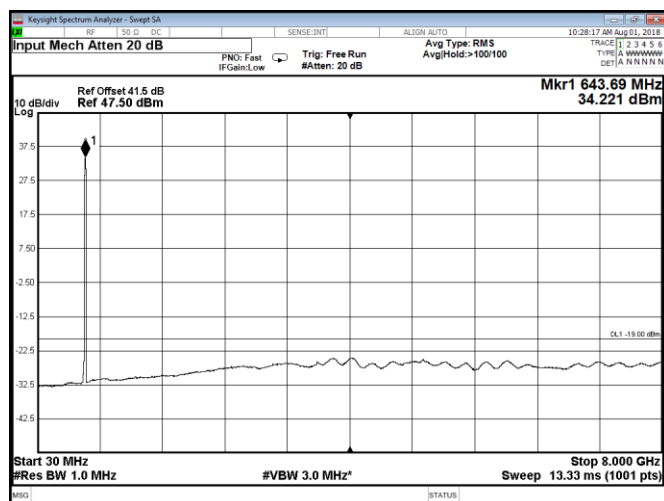
Figure 8.2-93: Conducted spurious emissions at Port A, QPSK, Band 71 high 15 MHz channel + IoT carrier
