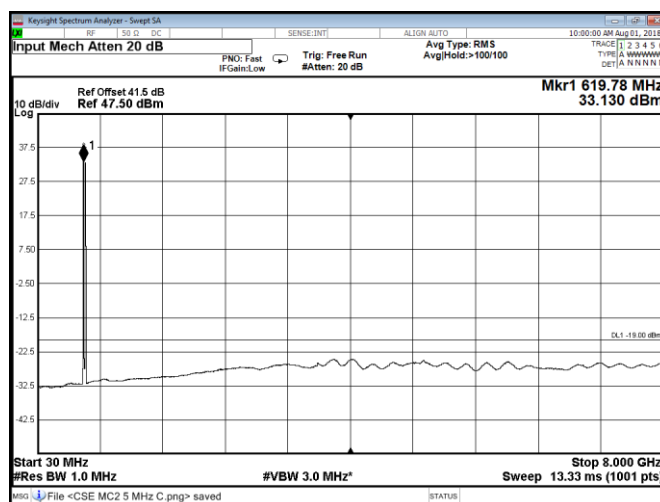
Figure 8.2-132: Conducted spurious emissions at Port D, QPSK, Band 71 multi carrier two 5 MHz channels
