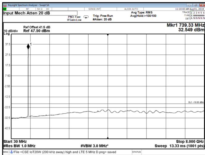
Figure 8.2-127: Conducted spurious emissions at Port C, Band 85A IoT carrier 200 kHz away from the upper band edge
