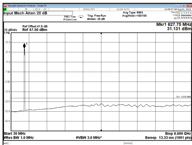
Figure 8.2-137: Conducted spurious emissions at Port A, QPSK, Band 71 multi carrier two 15 MHz channels
