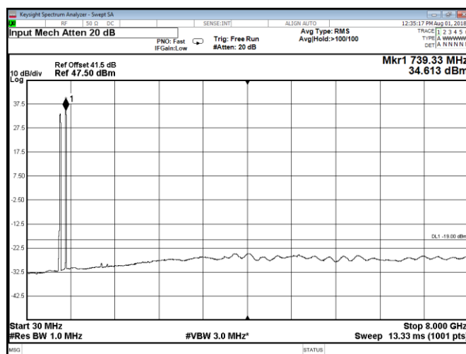
Figure 8.2-204: Conducted spurious emissions at Port D, QPSK, multi-band Band 71 20 MHz high channel and Band 85A 5 MHz high channel
