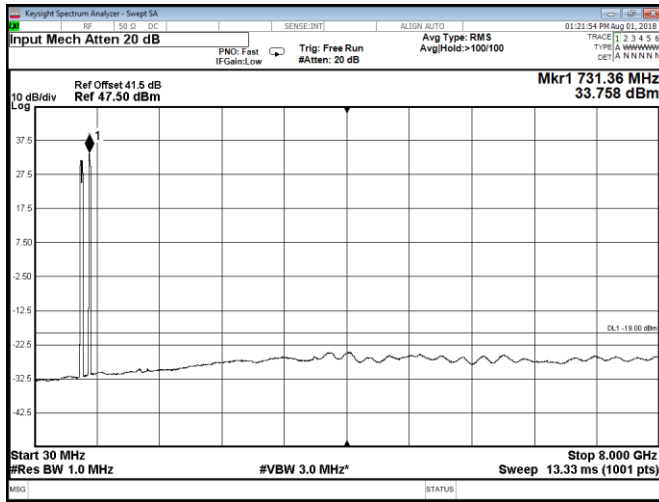
Figure 8.2-213: Conducted spurious emissions at Port A, QPSK, multi-band Band 71 two 15 MHz channels and Band 85A three 5 MHz channels
