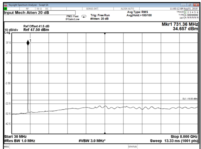
Figure 8.2-112: Conducted spurious emissions at Port D, QPSK, Band 85A low 10 MHz channel + IoT carrier
