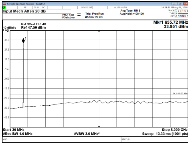
Figure 8.2-89: Conducted spurious emissions at Port A, QPSK, Band 71 mid 15 MHz channel + IoT carrier
