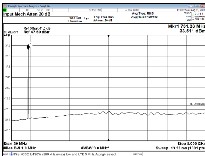
Figure 8.2-122: Conducted spurious emissions at Port B, Band 85A IoT carrier 200 kHz away from the lower band edge
