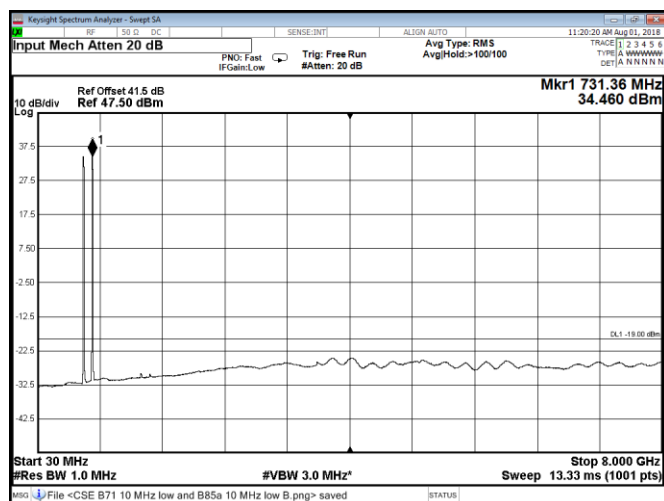
Figure 8.2-169: Conducted spurious emissions at Port A, QPSK, multi-band Band 71 10 MHz low channel and Band 85A 10 MHz low channel
