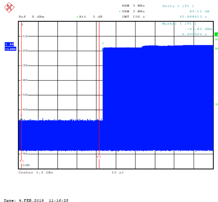
Figure 18 - Initial Channel Availability Check Time
