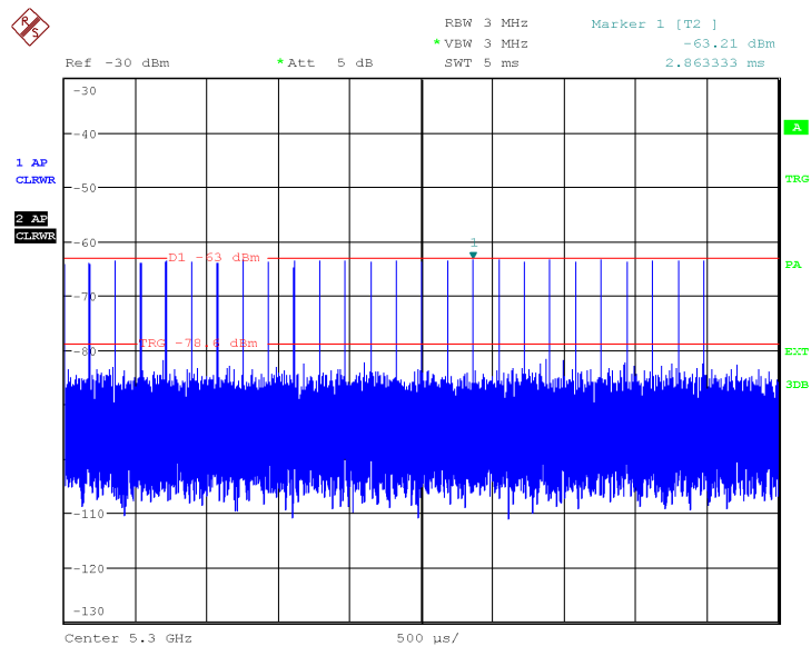
Figure 5 - Verification of Radar Type 1
