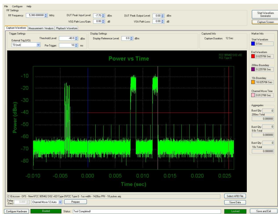
Figure 31 - Radar Test Signal Verification Plot
