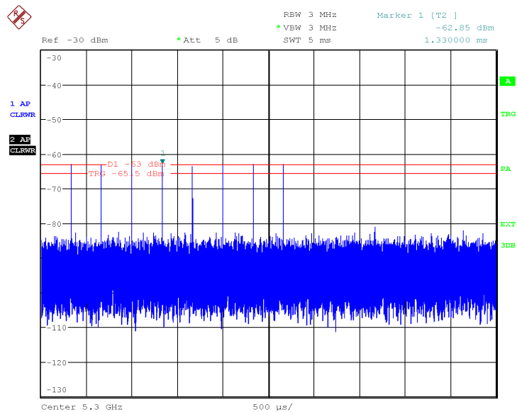
Figure 9 - Verification of Radar Type 5
