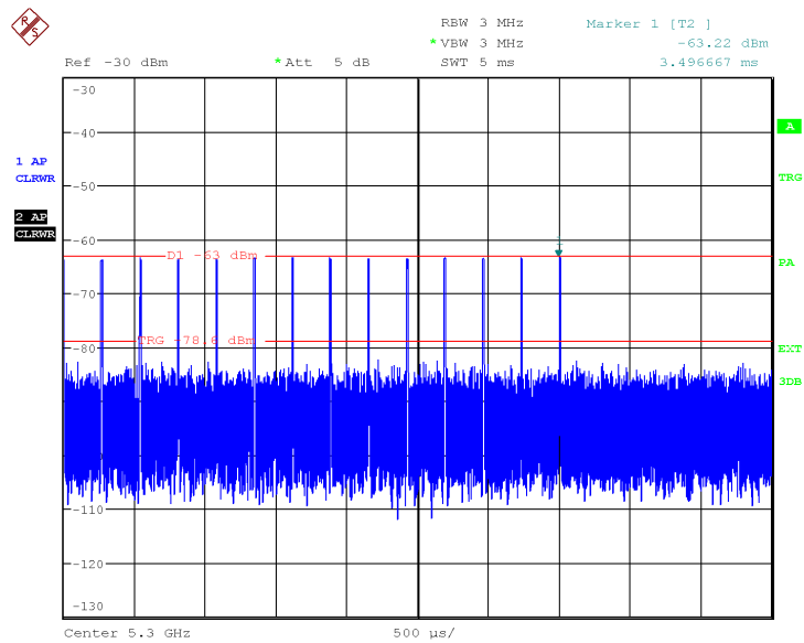
Figure 7 - Verification of Radar Type 3
