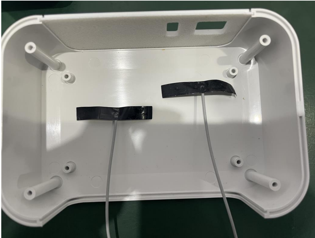
(CC2642R1F) BLE1&BLE2 Antenna-3
