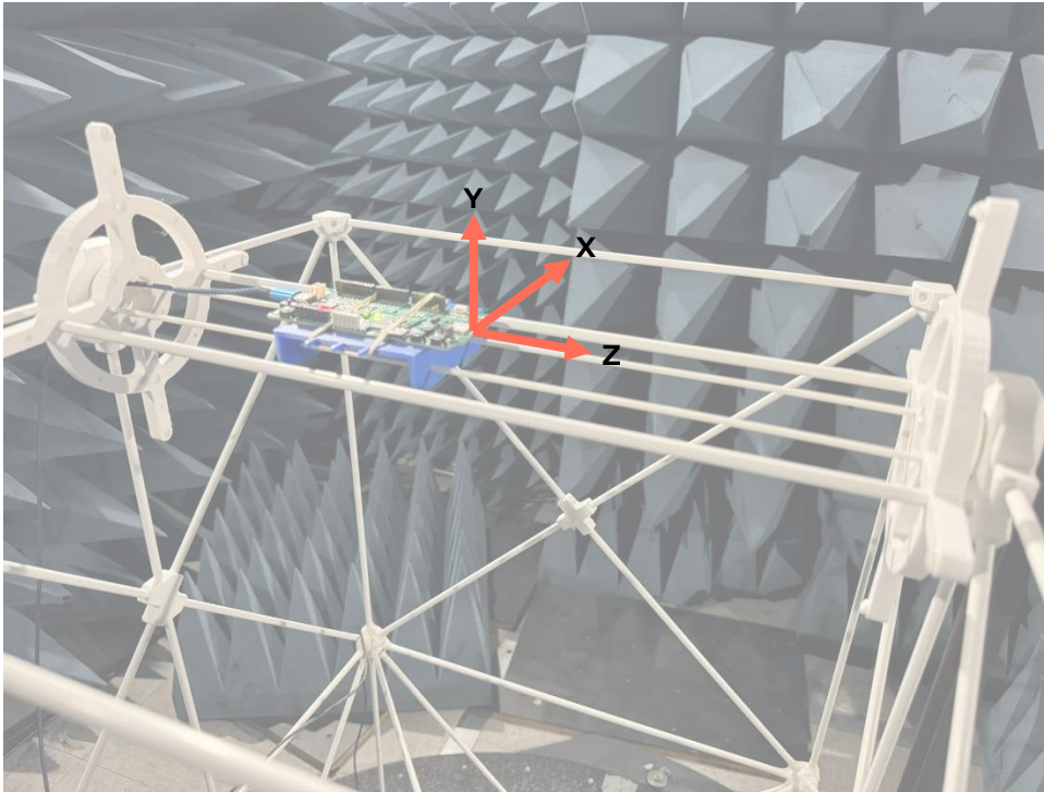
Figure 2: NORA-W3x6 patch antenna on EVK mounted in test chamber
