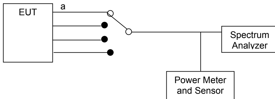
Measurement setup for Peak Power Spectral Density
