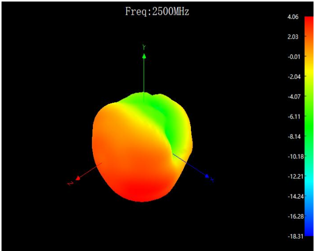
2500MHz 3D-Total Pattern
