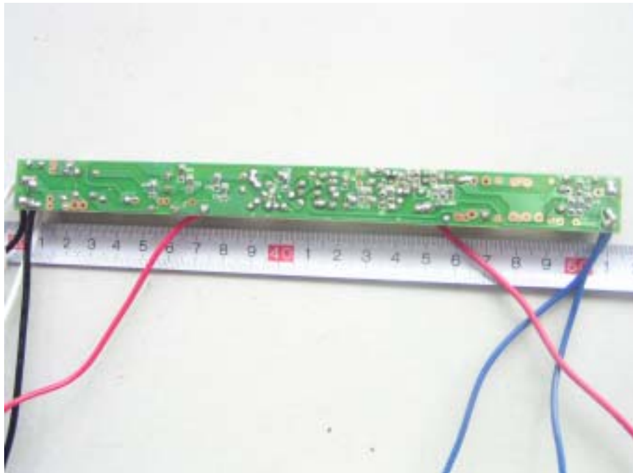
EDFT5-128L-MCO: EUT-PCB Bottom View
