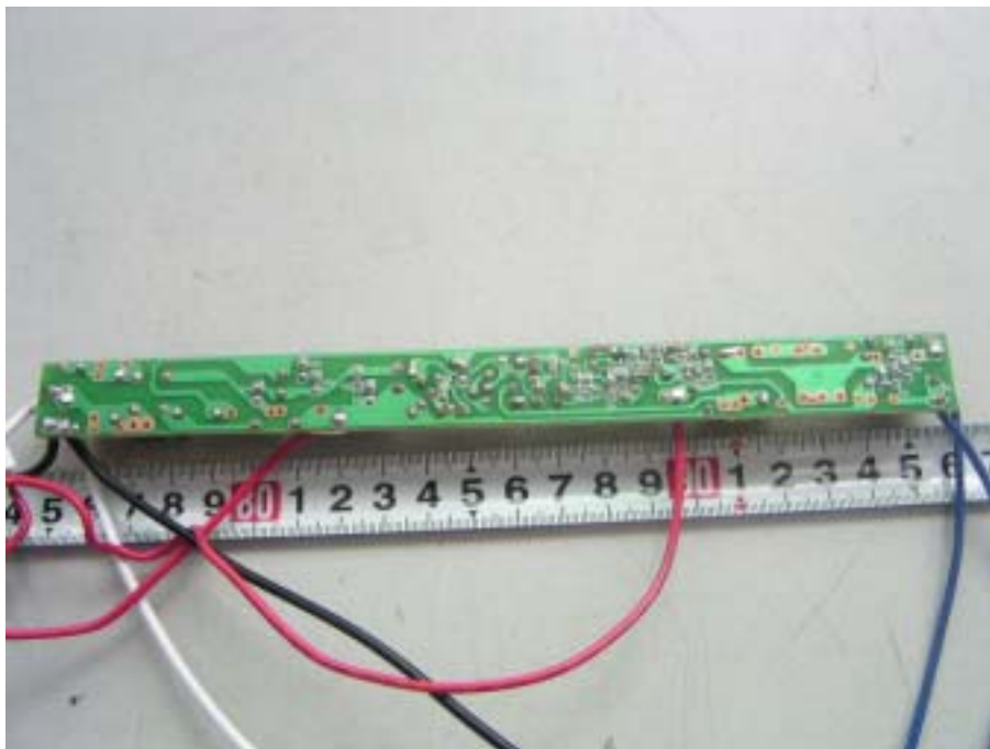
EDFT5-124L-MAO: EUT-PCB Bottom View
