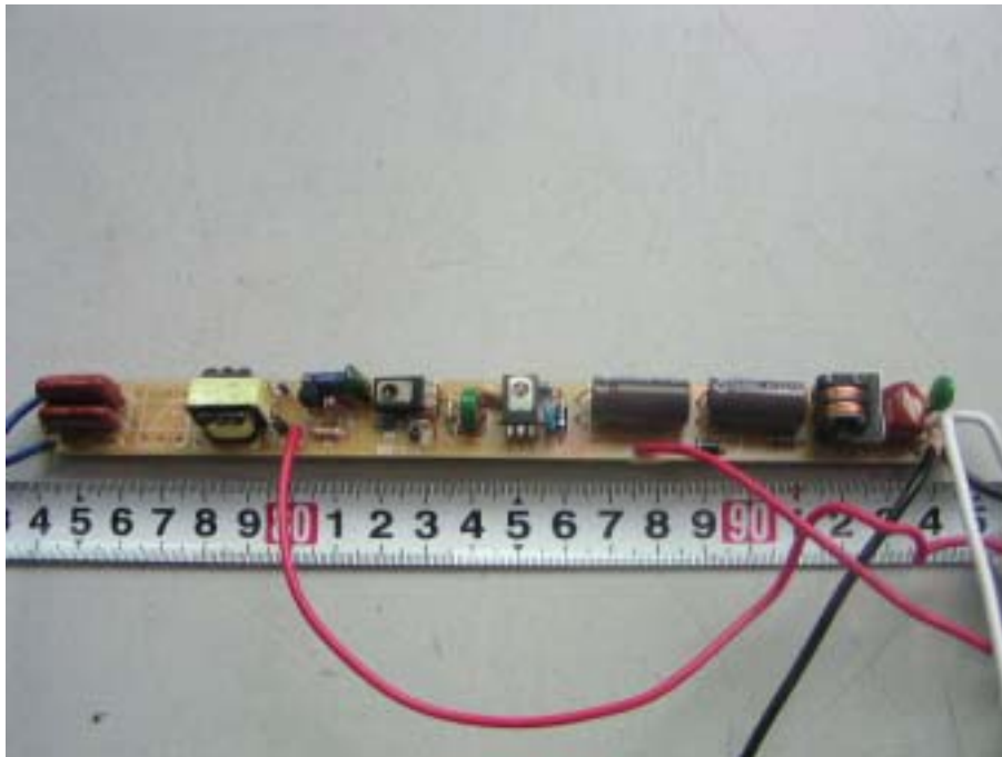
EDFT5-124L-MAO: EUT-PCB Top View
