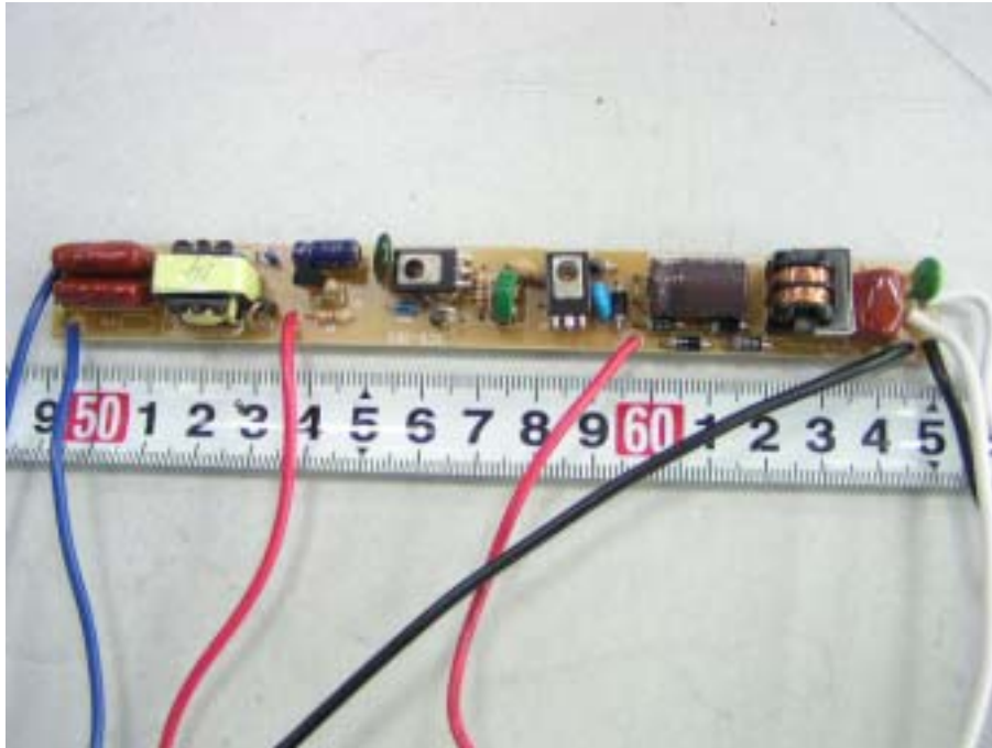
EDFT5-113L-MFO: EUT-PCB Top View
