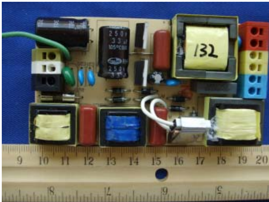
EBC09-132UH-PM2 –Components View
