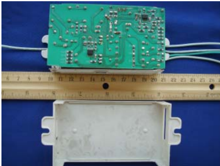
EBC09-132UH-PM2 – Uncovered View
