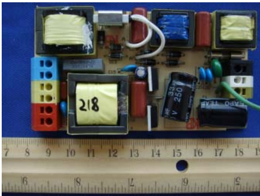
EBU2U-218UH-PM2 –Components View
