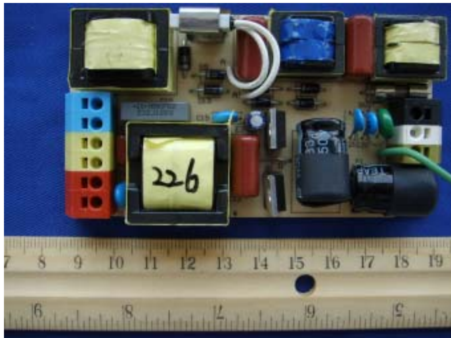
EBU2U-226UH-PM2 –Components View
