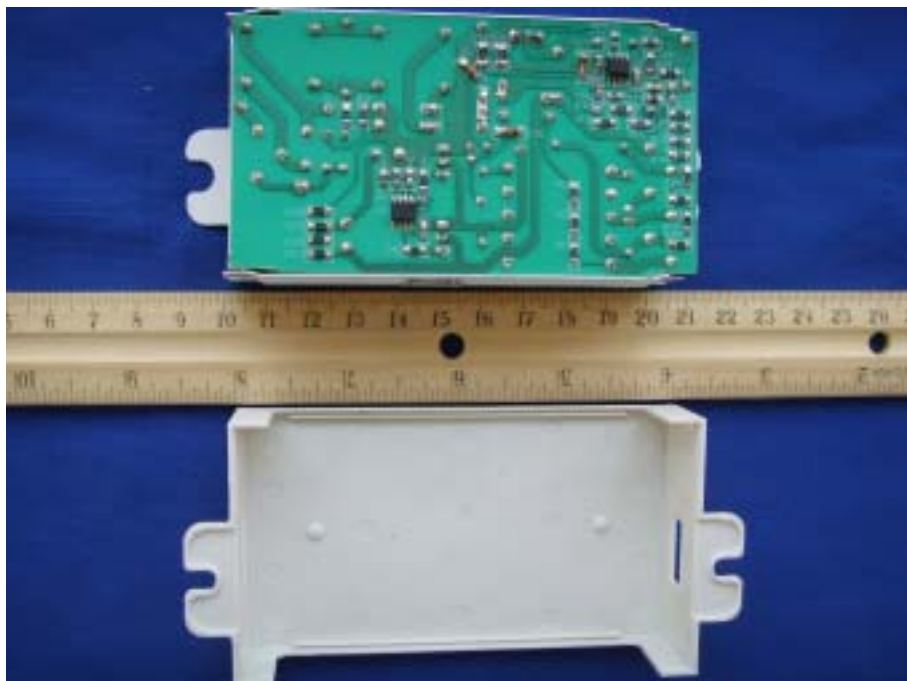
EBU2U-226UH-PM2 – Uncovered View
