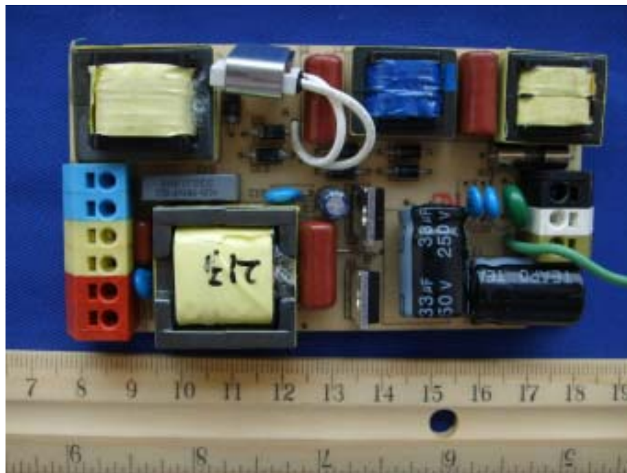
EBU2U-213UH-PM2 –Components View
