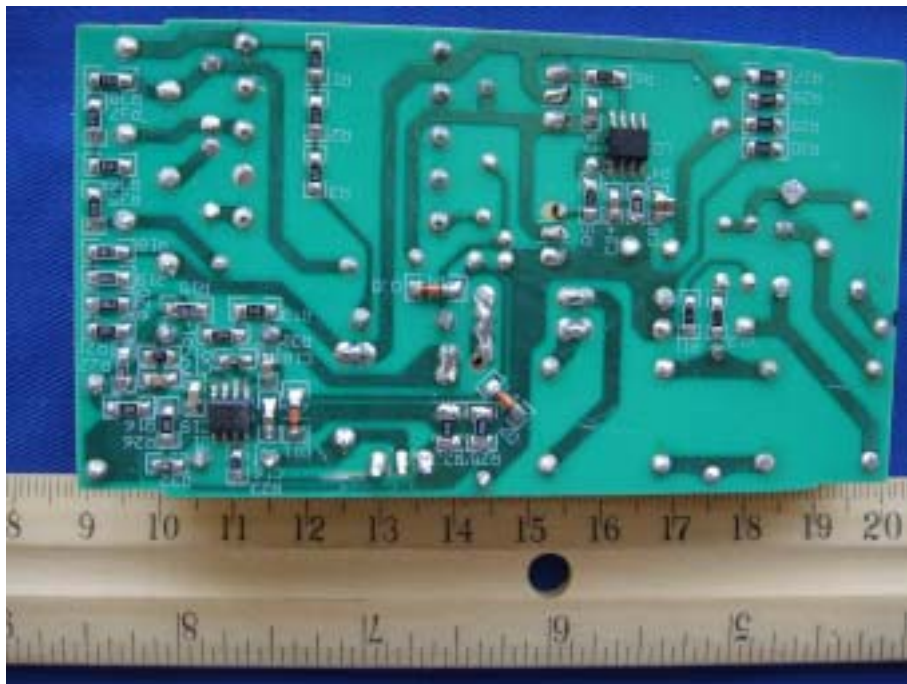
EBC09-132UH-PM2–Solder View
