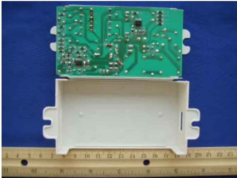
EBU2U-218UH-PM2 – Uncovered View
