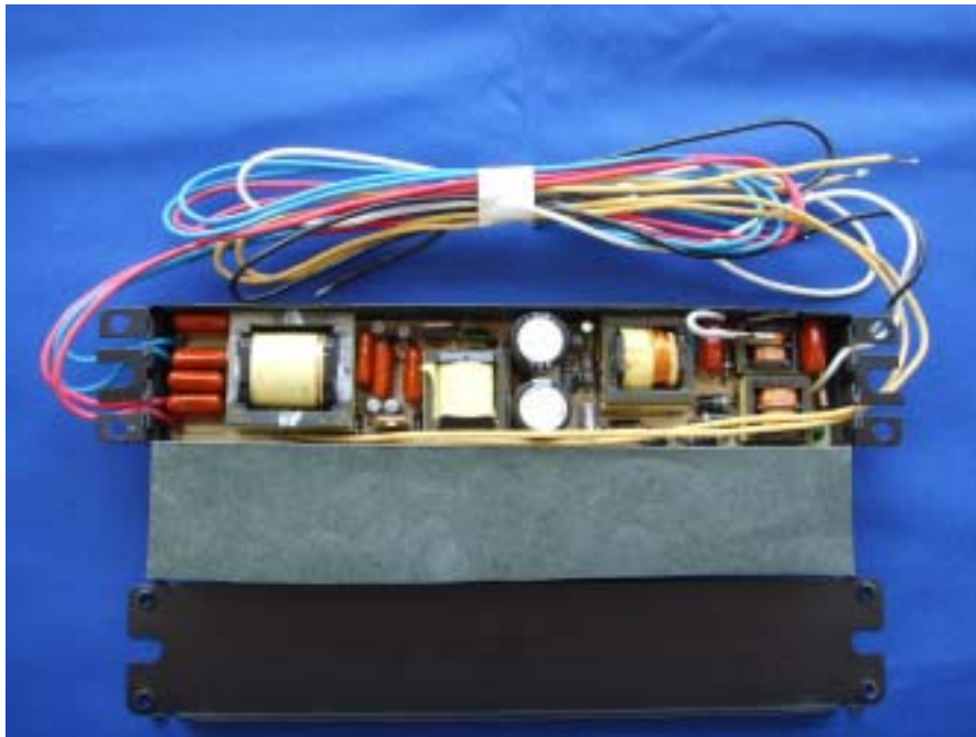
EBT08-432UH-MS1-00 – Uncovered View
