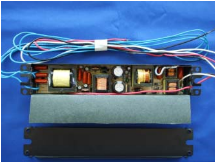
EBT08-332UH-MS1-00 – Uncovered View
