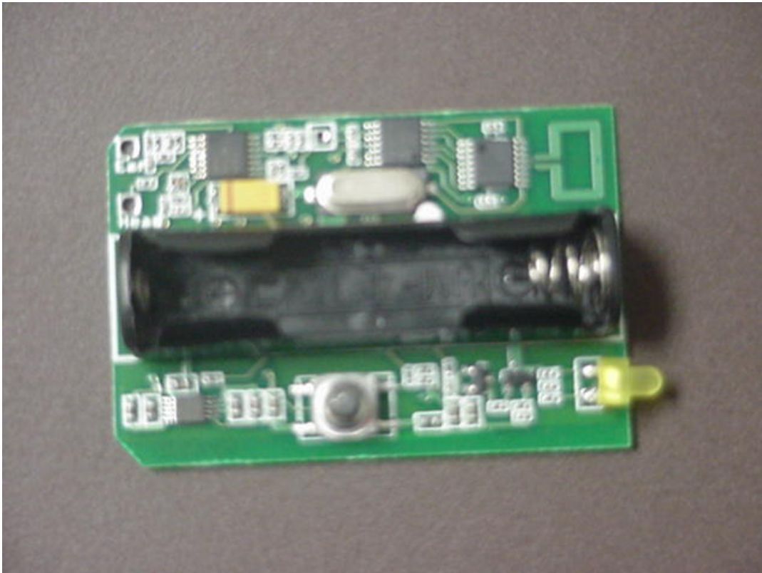
EUT with Battery Holder Present (Next photo provides better detail.)
