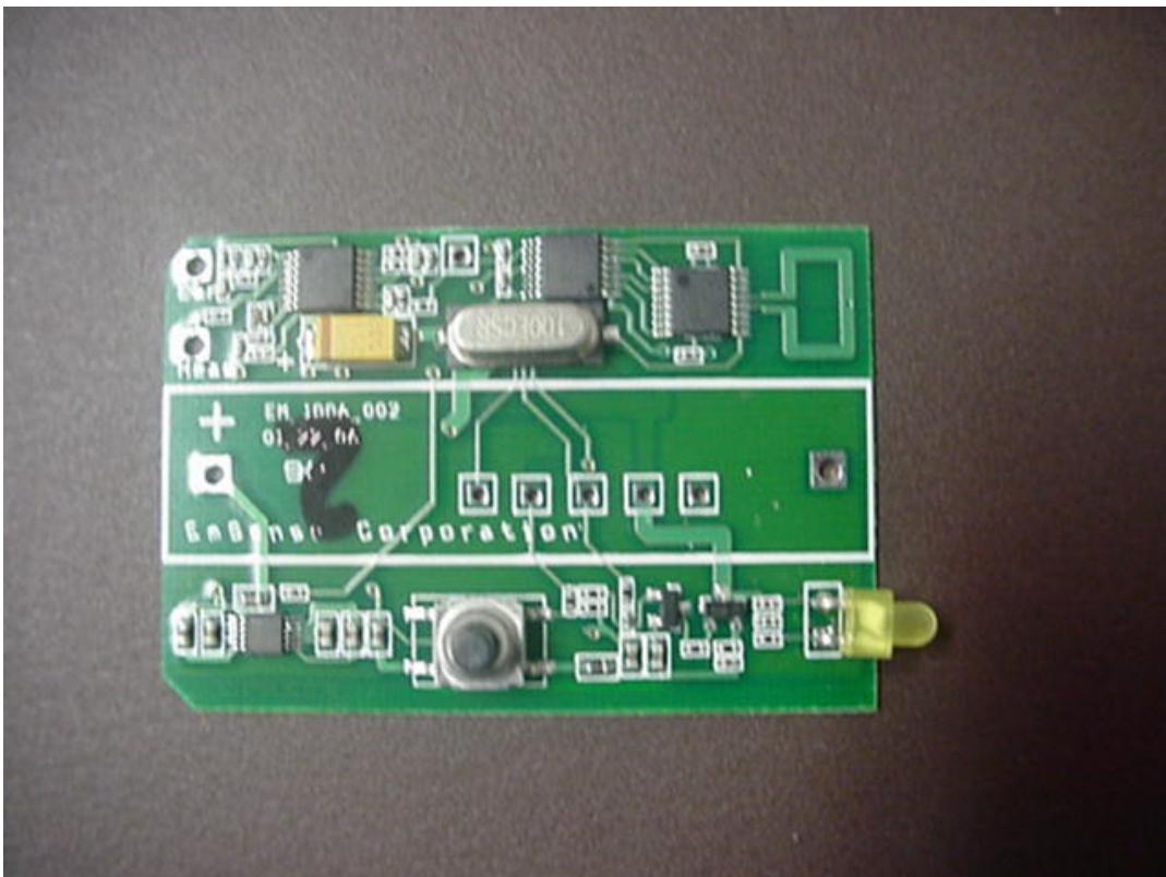
EUT PCB Top with Battery Holder Removed (Antenna is the thick rectangular trace visible on upper right of PCB.)
