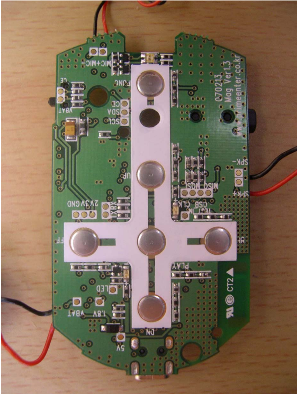
&lt;Photograph 3: Main Board Rear View&gt;
