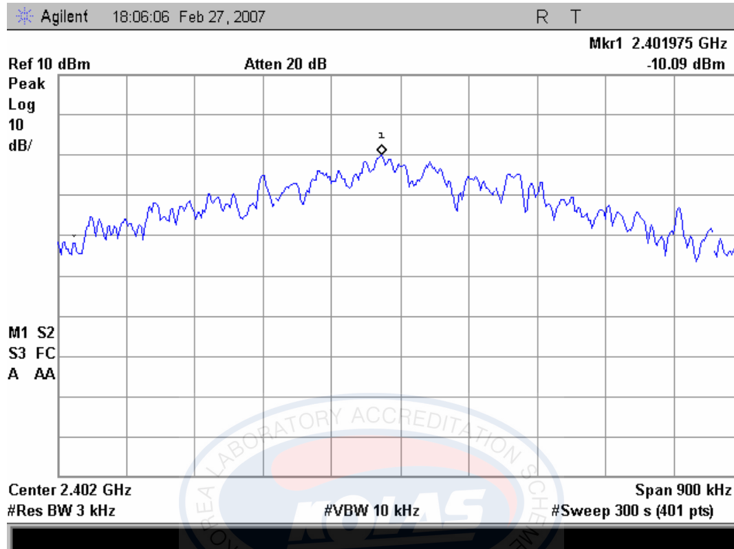
Figure 9. Plot of the Peak Power Spectral Density (Conducted)
