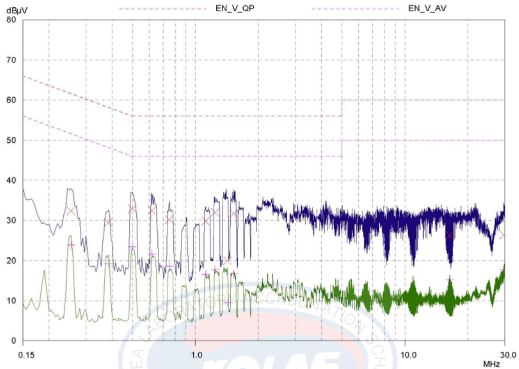
Figure 10. Plot of the Conducted Emissions
