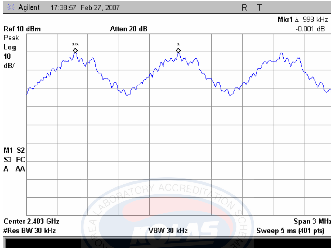
Figure 2. Plot of the Carrier Frequency Separation (Conducted)
