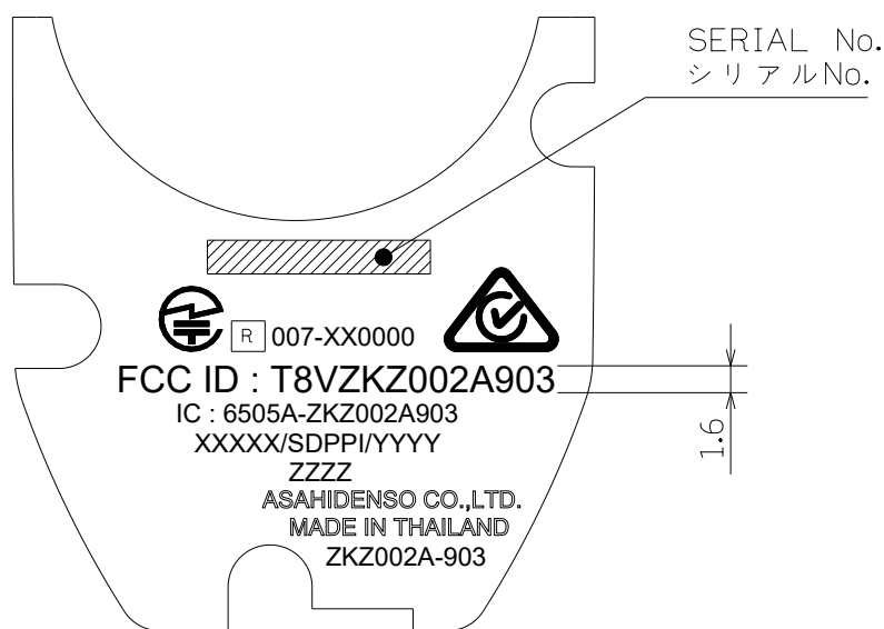
DETAIL OF B (2 : 1)
