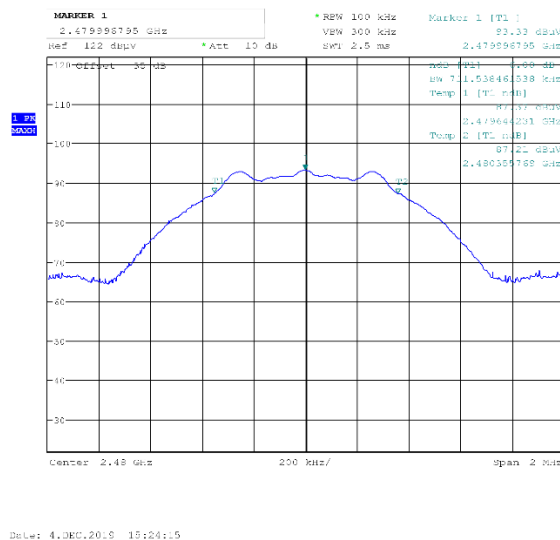
Figure 8.7-3: PSD plot on High channel
