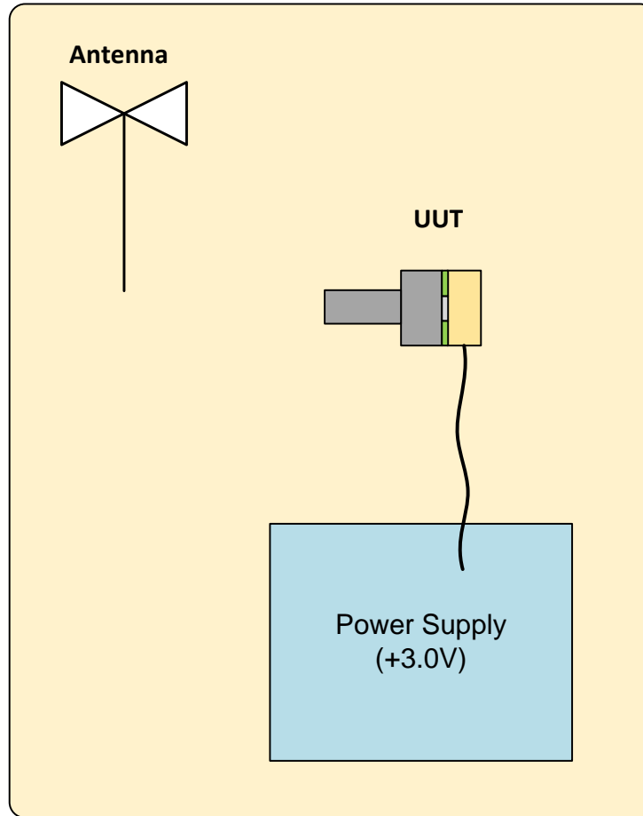
Figure 3.6-1: Setup diagram
