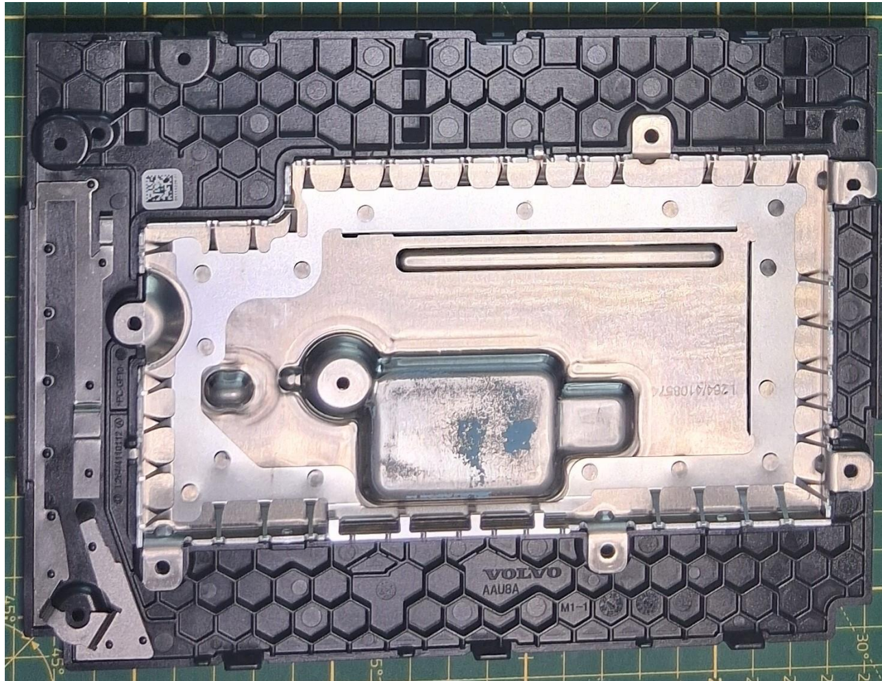
Housing inside
