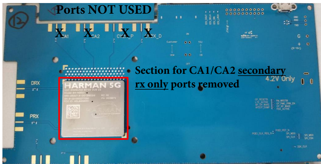
Figure 1.1-2 : SA-N9001 CUS D1
