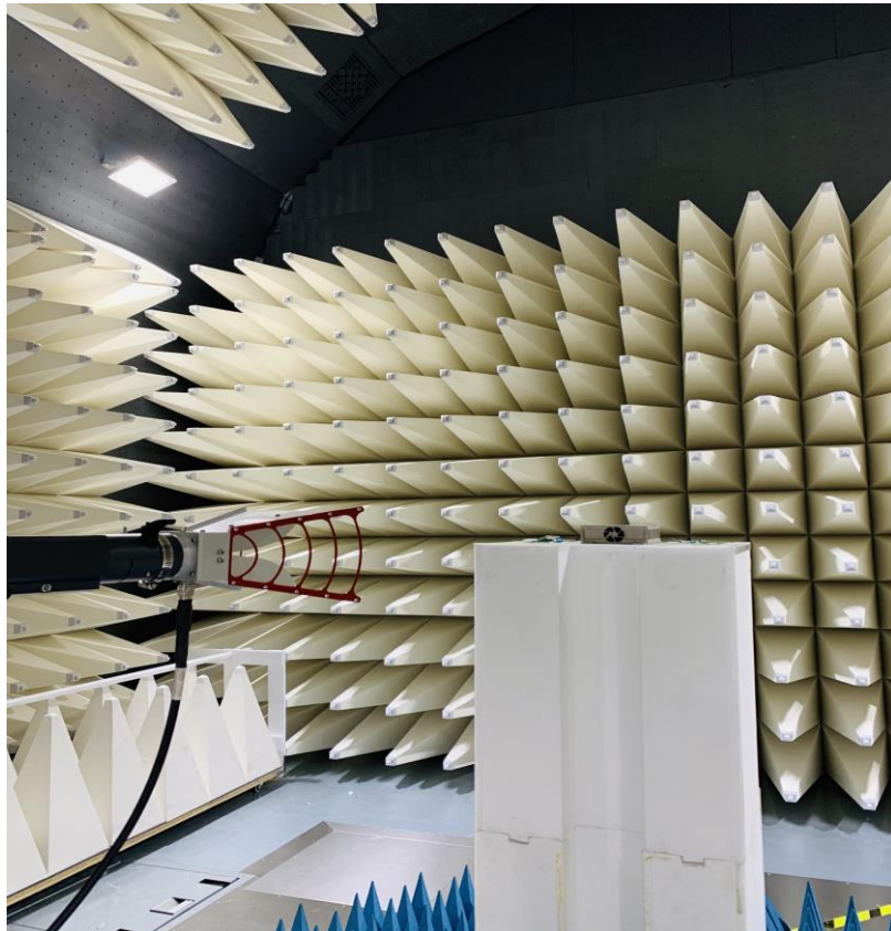
Figure3. Radiated Setup – High Range
