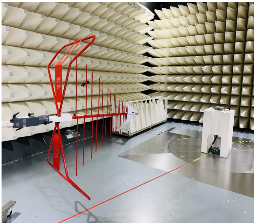
Figure D4. Radiated Setup – Low Range
