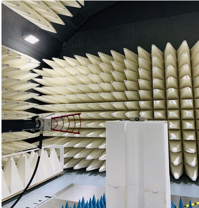
FigureC3. Radiated Setup – High Range
