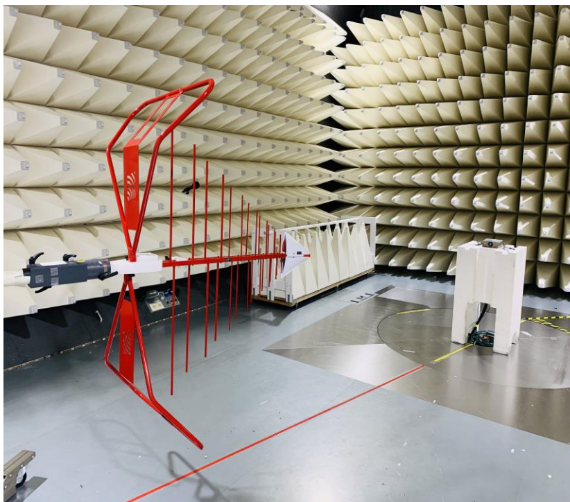
Figure C4. Radiated Setup – Low Range
