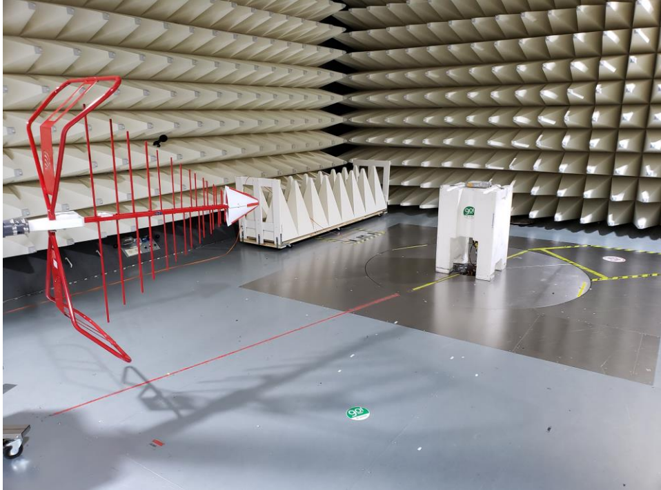
Figure B5. Low Range Radiated Emission test setup
