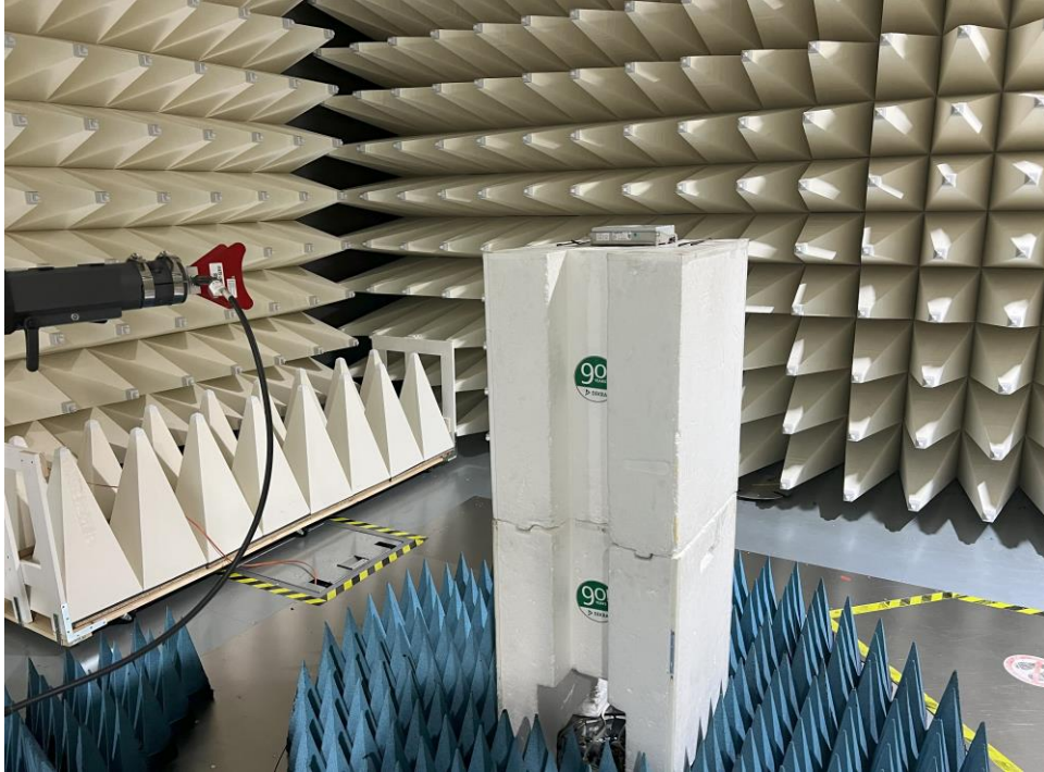
Figure B7. High Range Radiated Emission test setup 1
