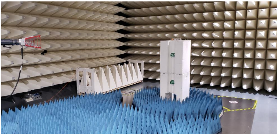
Figure B6. Low Range Radiated Emission test setup
