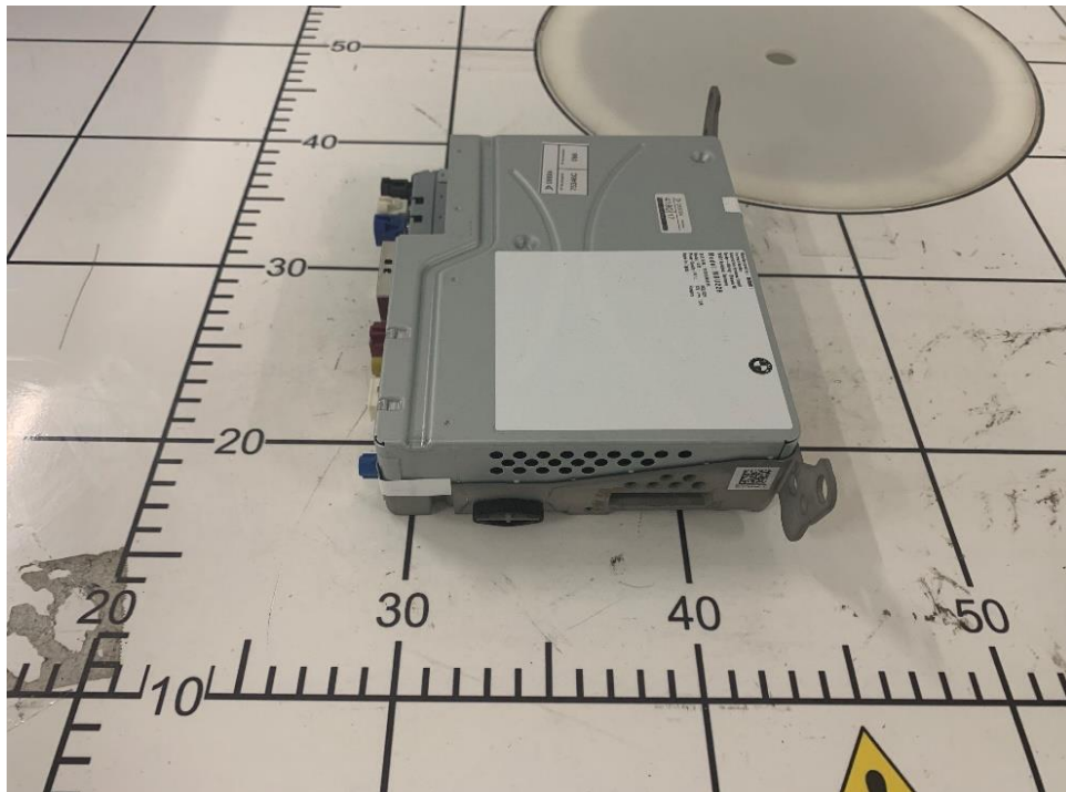
Figure C3. Side View of DUT
