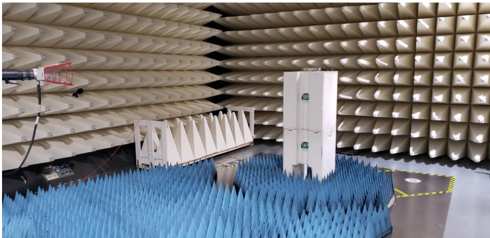
Figure C6. High Range Radiated Emission test setup 1
