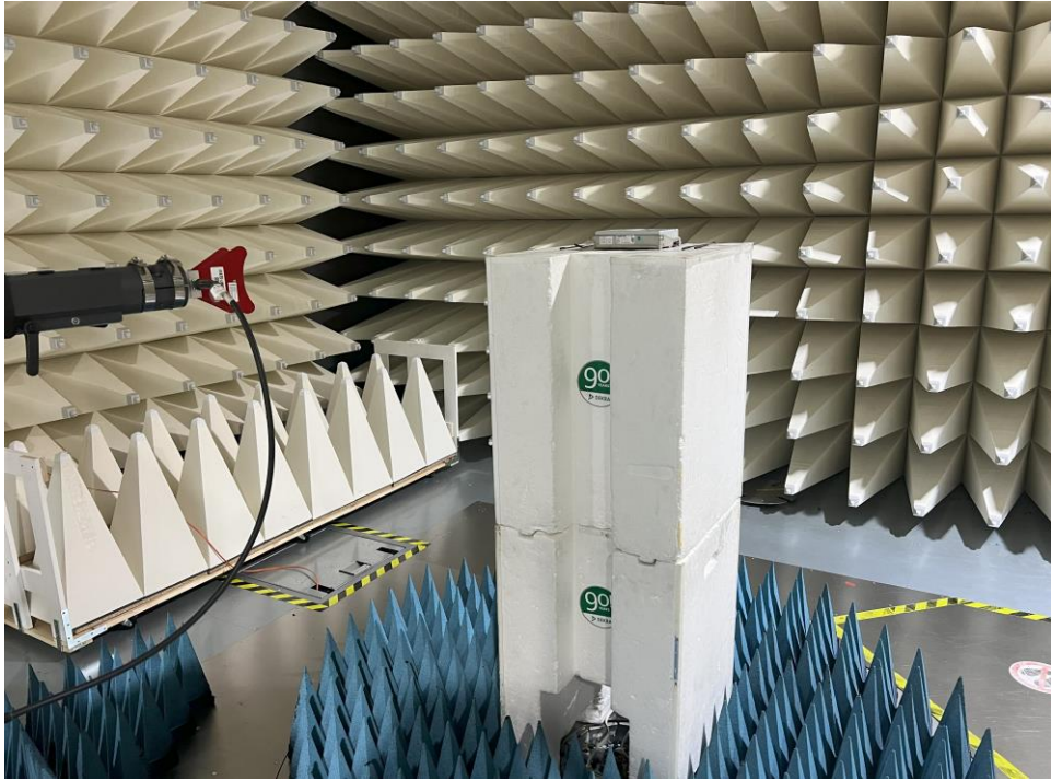
Figure C7. High Range Radiated Emission test setup 2
