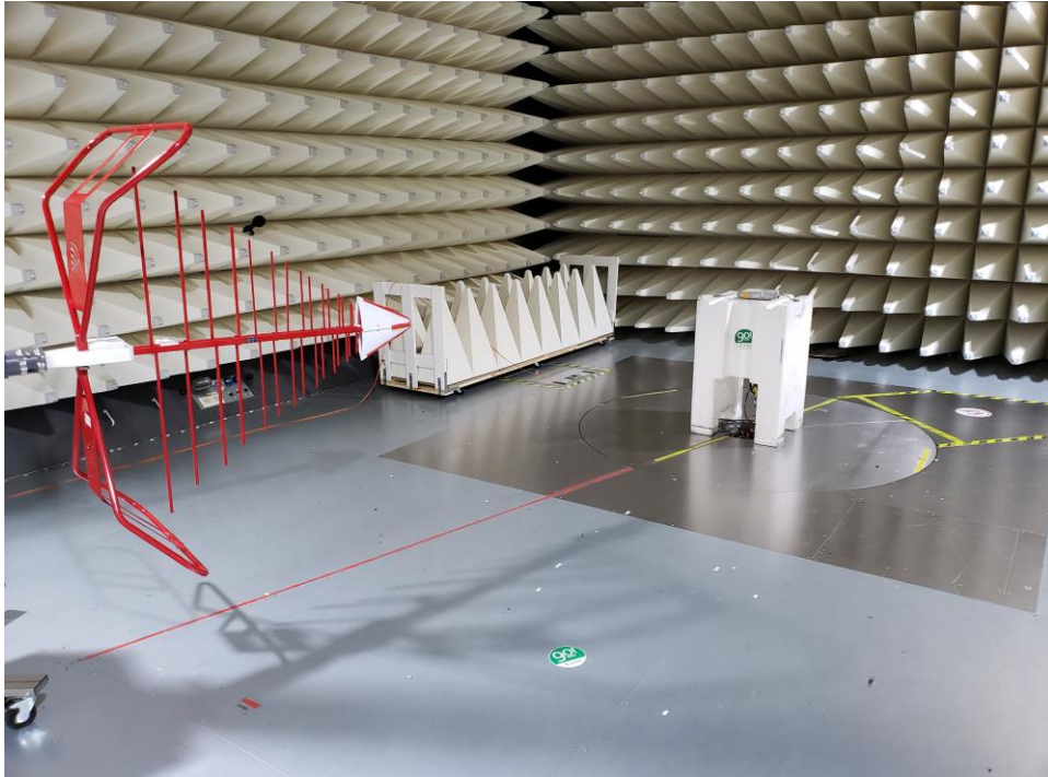
Figure C5. Low Range Radiated Emission test setup
