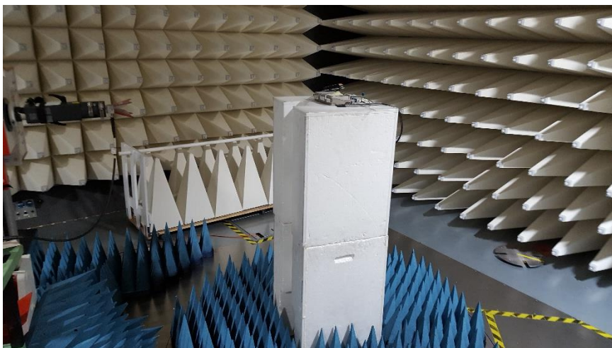
Figure B6. High Range Radiated Emission test setup 18-40GHz
