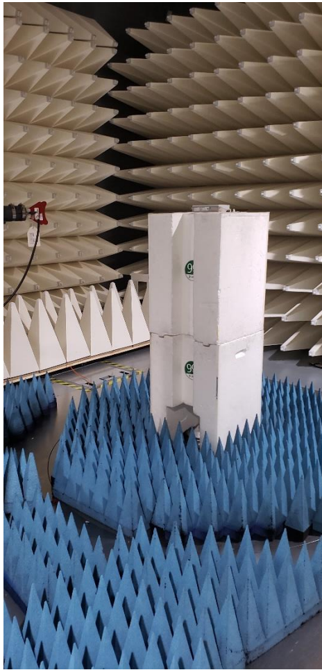
Figure B7. High Range Radiated Emission test setup 18-40 GHz
