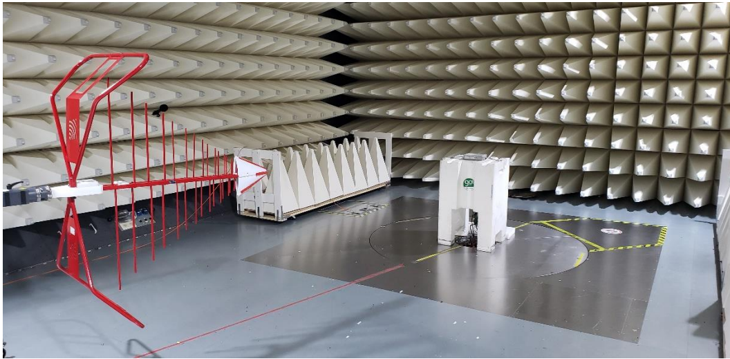
Figure B5. Low Range Radiated Emission test setup
