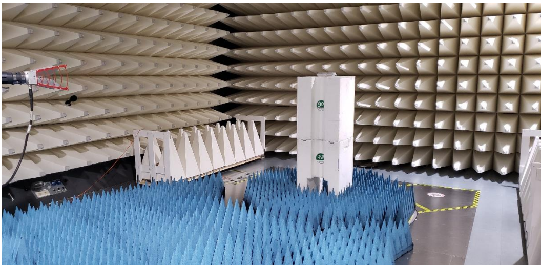
Figure C6. High Range Radiated Emission test setup
