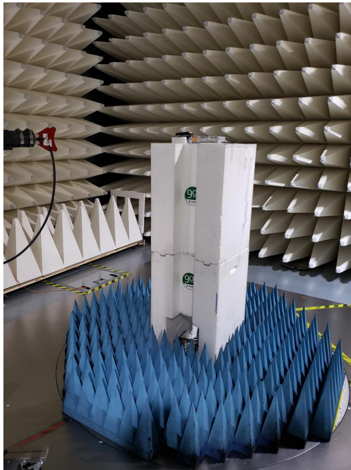
Figure B7. High Range Radiated Emission test setup 2
