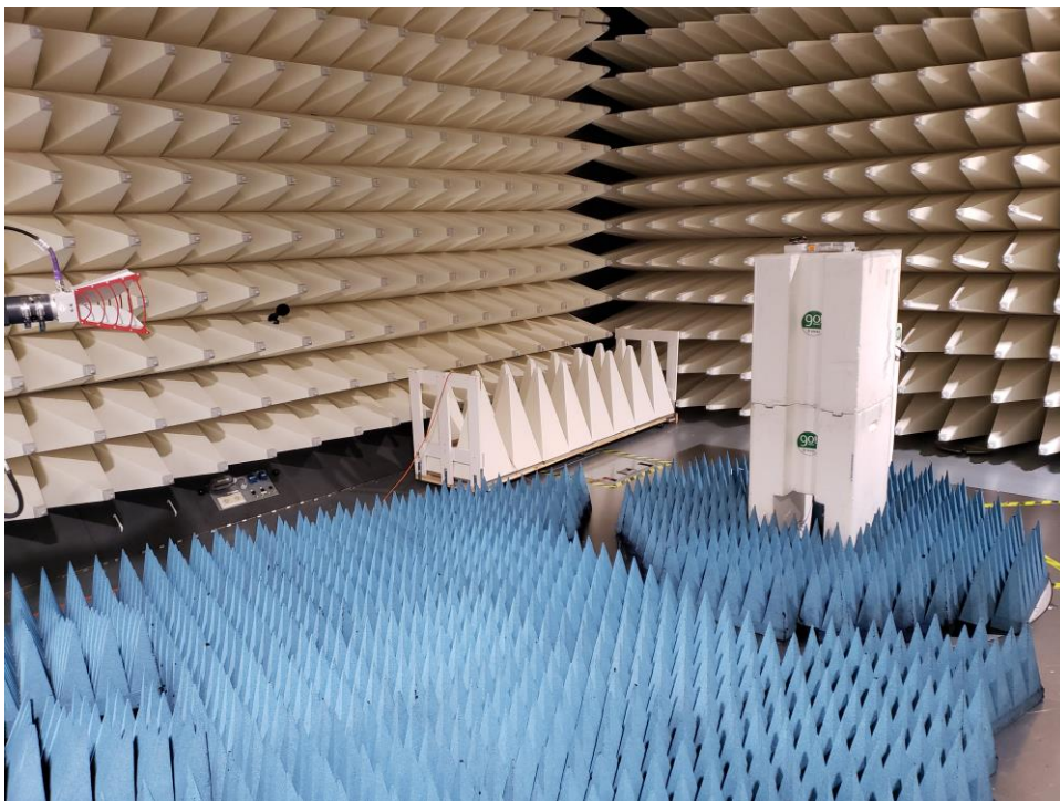
Figure B6. High Range Radiated Emission test setup 1
