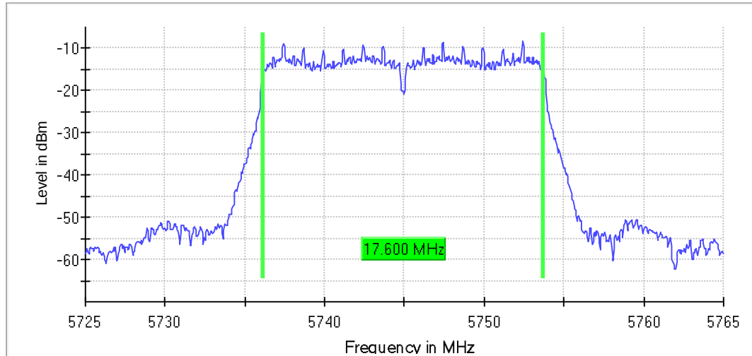
6 dB Bandwidth
