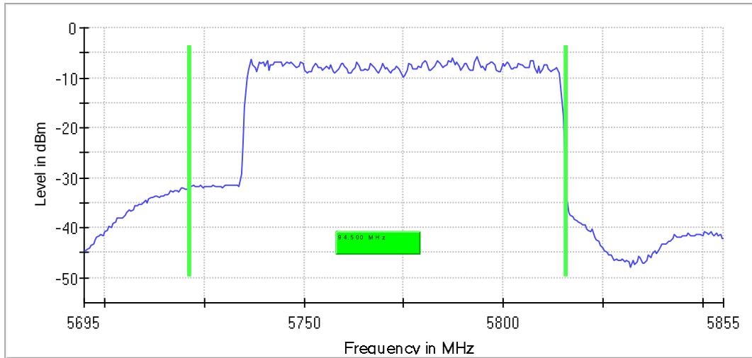
26 dB Bandwidth
