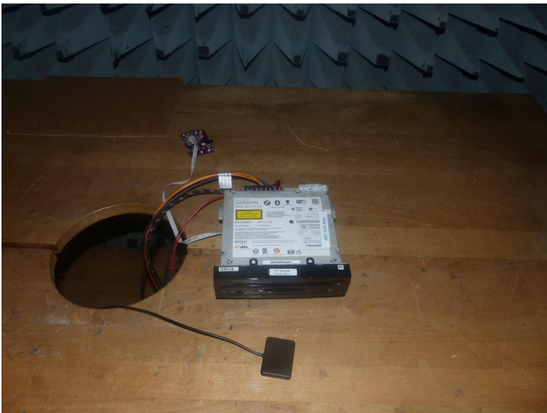
Photo 2: Radiated test setup for H-Field
