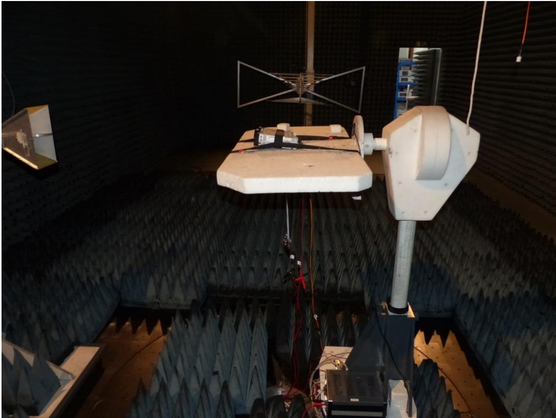
Photo 5: Radiated test setup for 1GHz – 25GHz.
