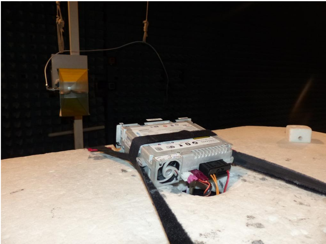
Photo 6: Radiated test setup for 1GHz – 25GHz
