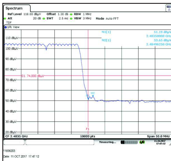
Upper Band Edge Peak Hopping
