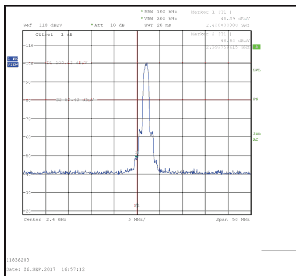
Lower Band Edge Peak Static
