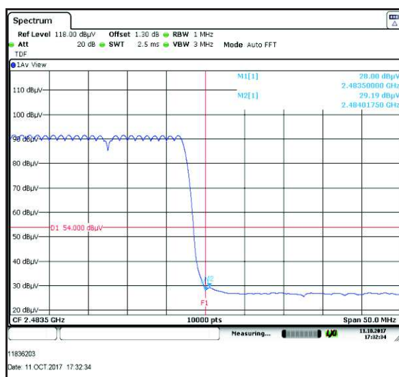
Upper Band Edge Average Hopping
