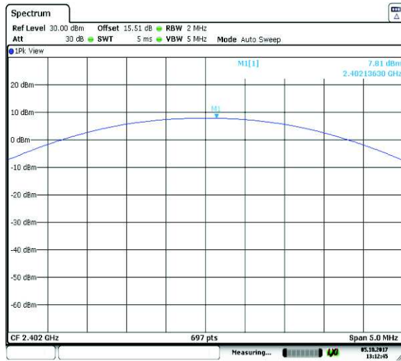
Bottom Channel
