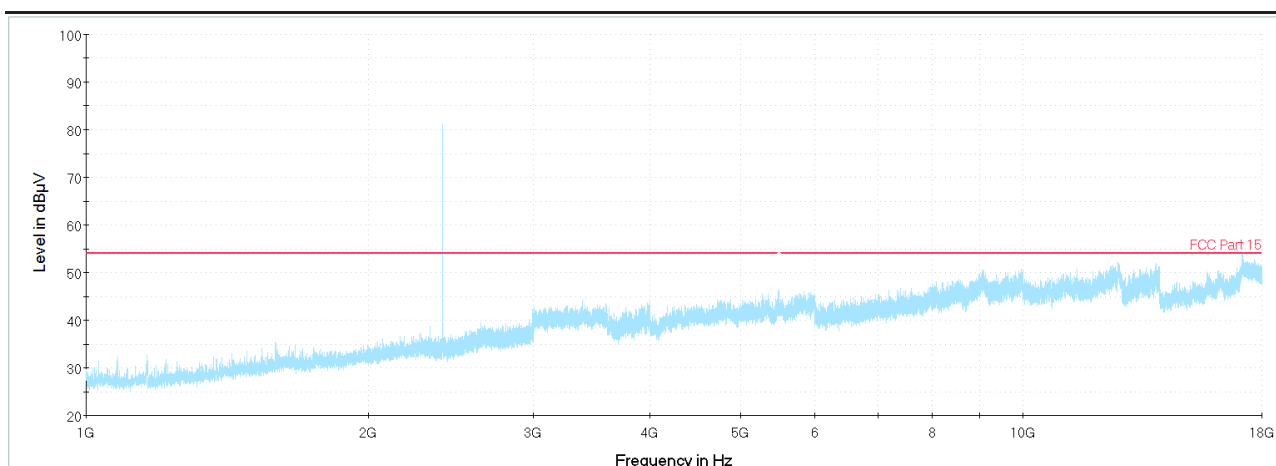
Bottom channel
