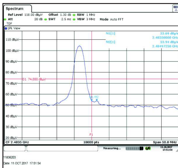
Upper Band Edge Peak Static
