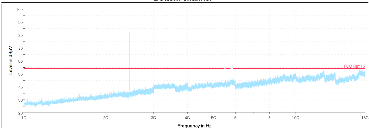
Bottom channel
