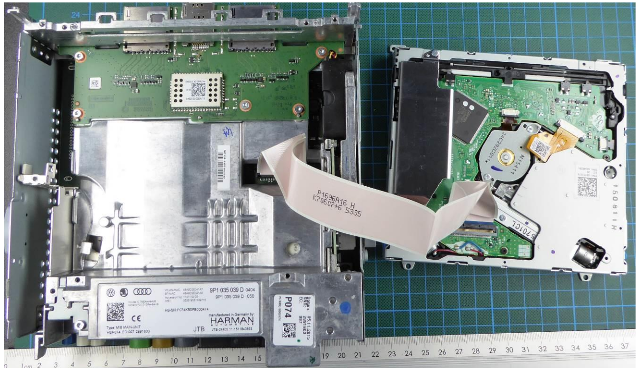
160090_23. jpg: EUT – Main Unit – Inside view with cd drive outside
