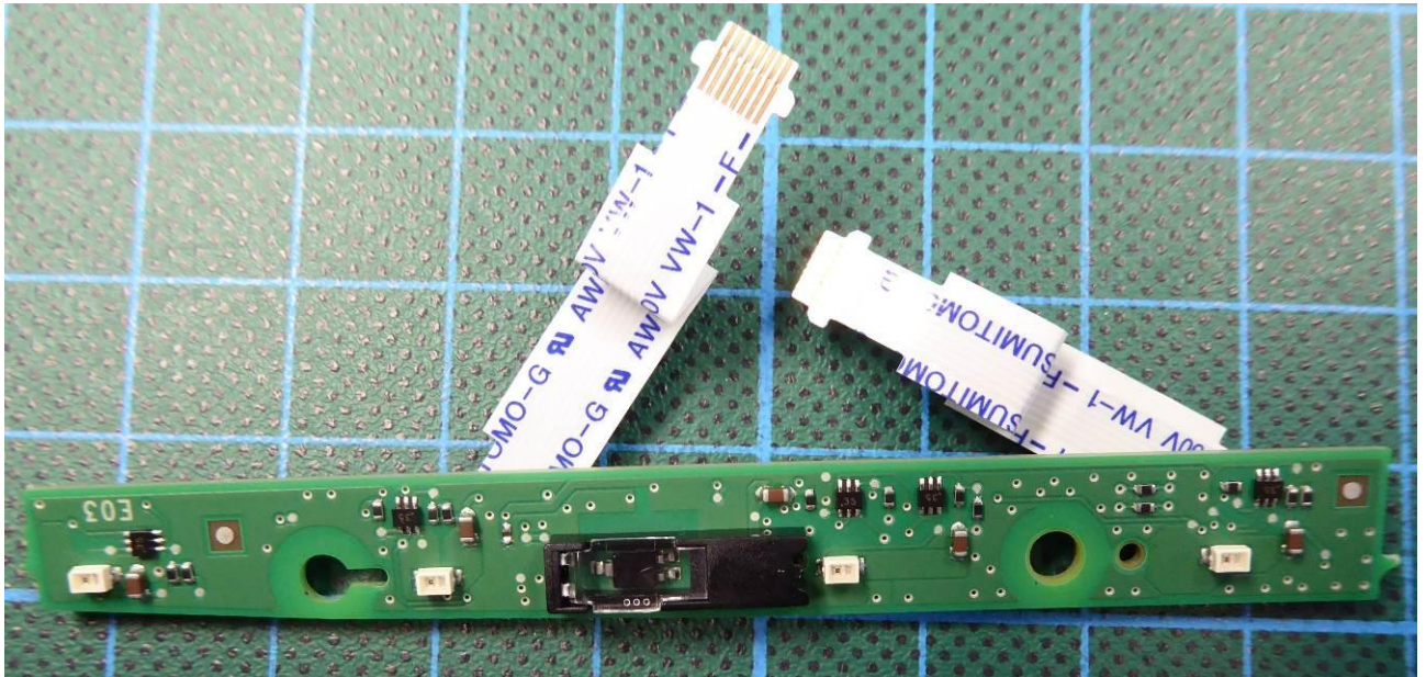
160090_15. jpg: EUT – Front panel – “LED” PCB bottom view
