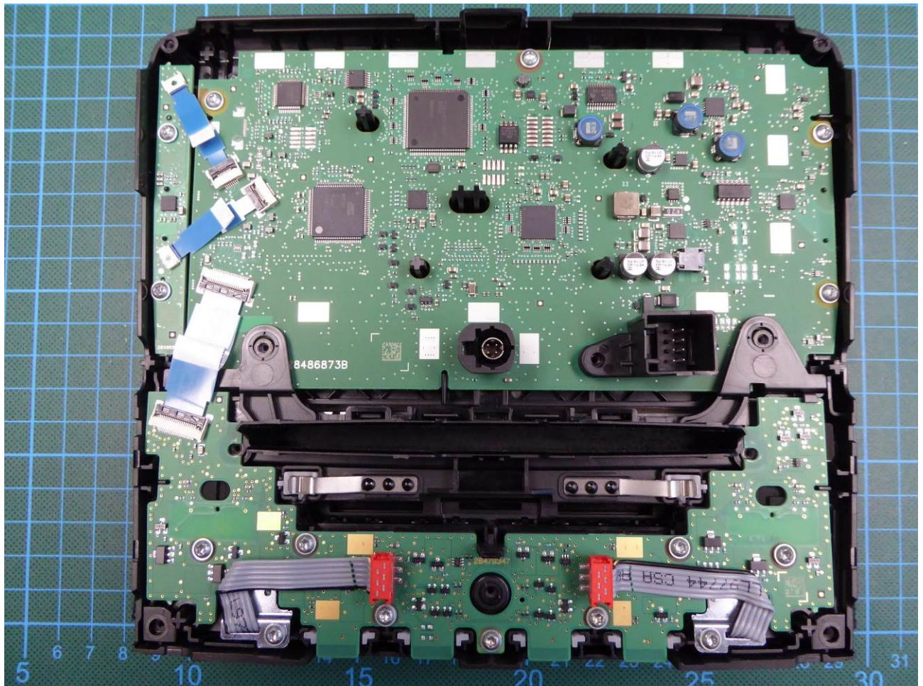
160090_08. jpg: EUT – Front panel inside view
