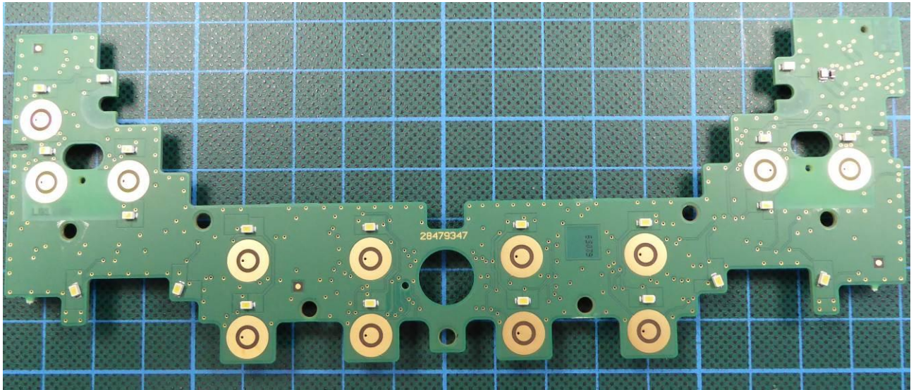
160090_13. jpg: EUT – Front panel – “Button” PCB bottom view
