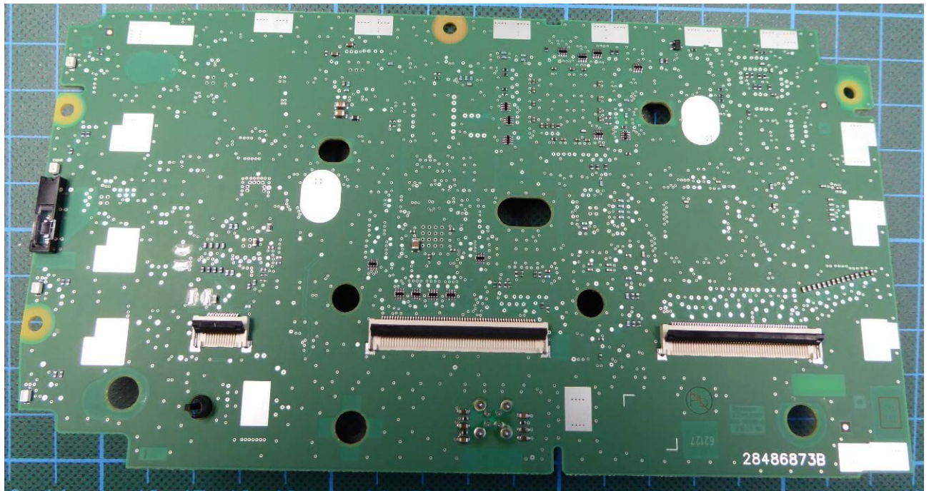
160090_11. jpg: EUT – Front panel – Main PCB bottom view
