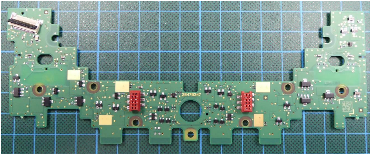
160090_12. jpg: EUT – Front panel – “Button” PCB top view
