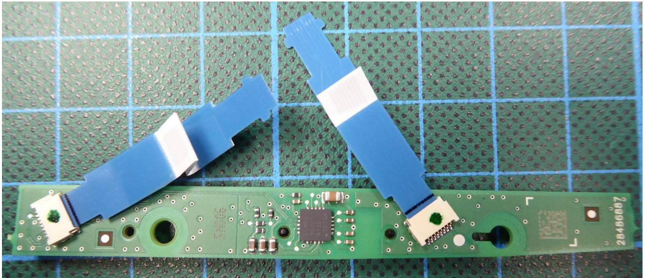
160090_14. jpg: EUT – Front panel – “LED” PCB top view
