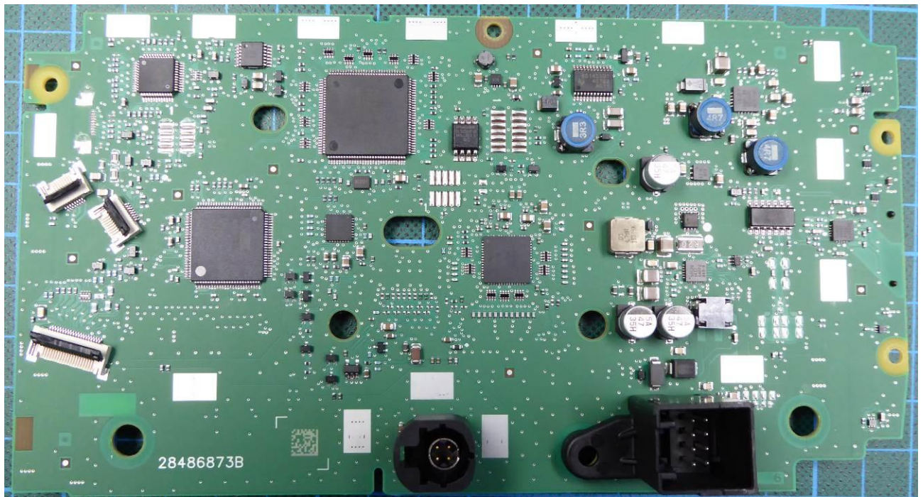
160090_10. jpg: EUT – Front panel – Main PCB top view
