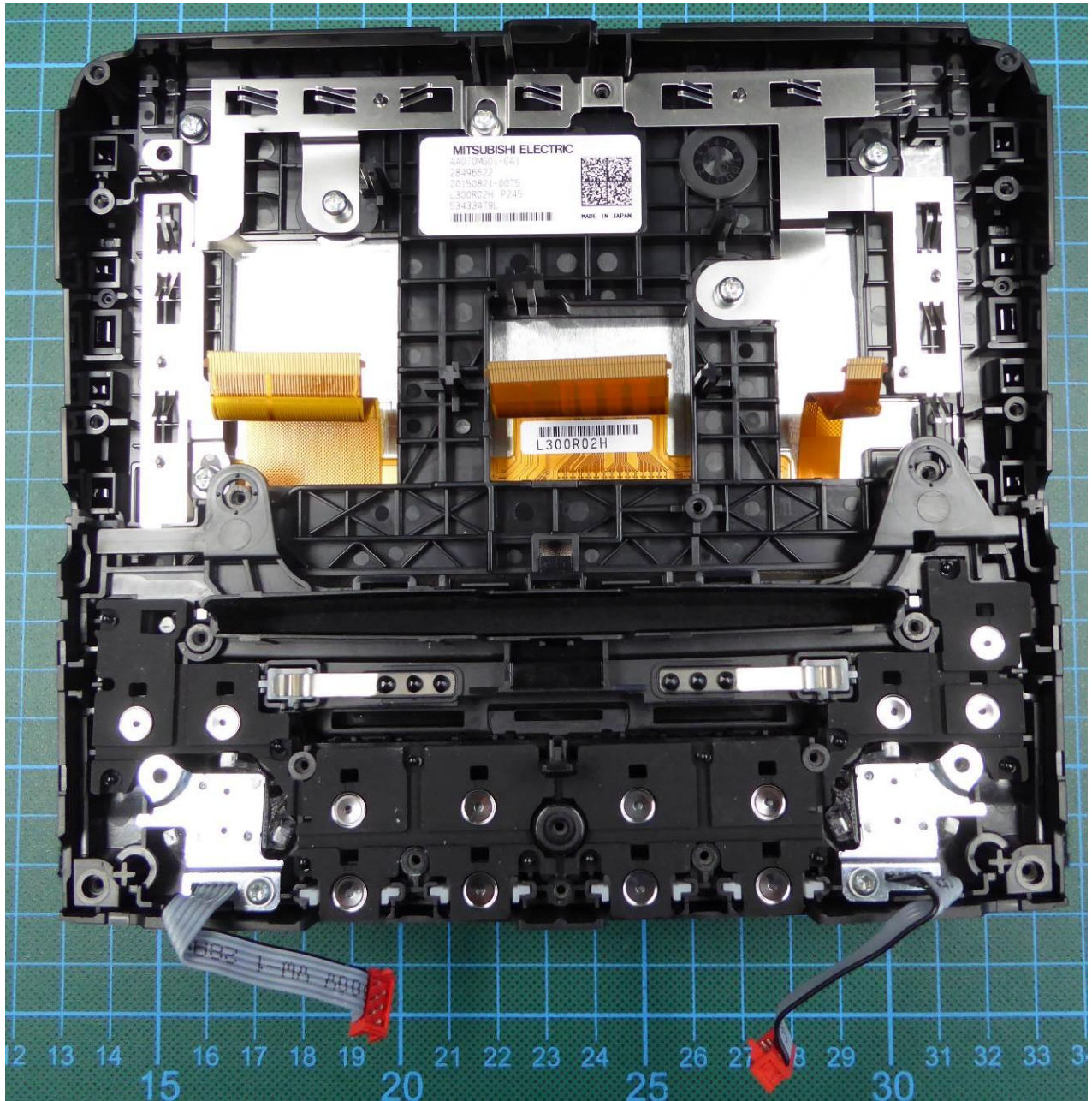
160090_09. jpg: EUT – Front panel without PCBs
