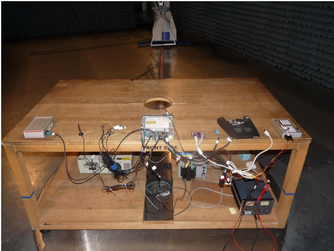
Photo 2: Test setup for radiated measurements, rear view (Enclosure, semi-anechoic chamber, 30 MHz to 1 GHz, intentional radiator §15)
