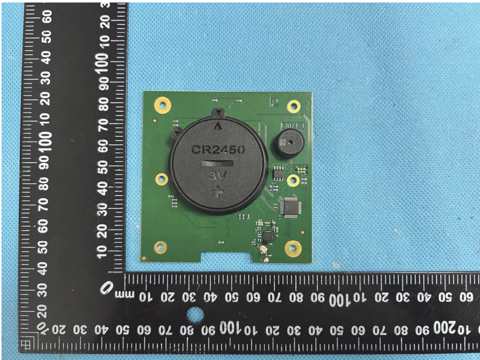
Solder Board-Component View 1
