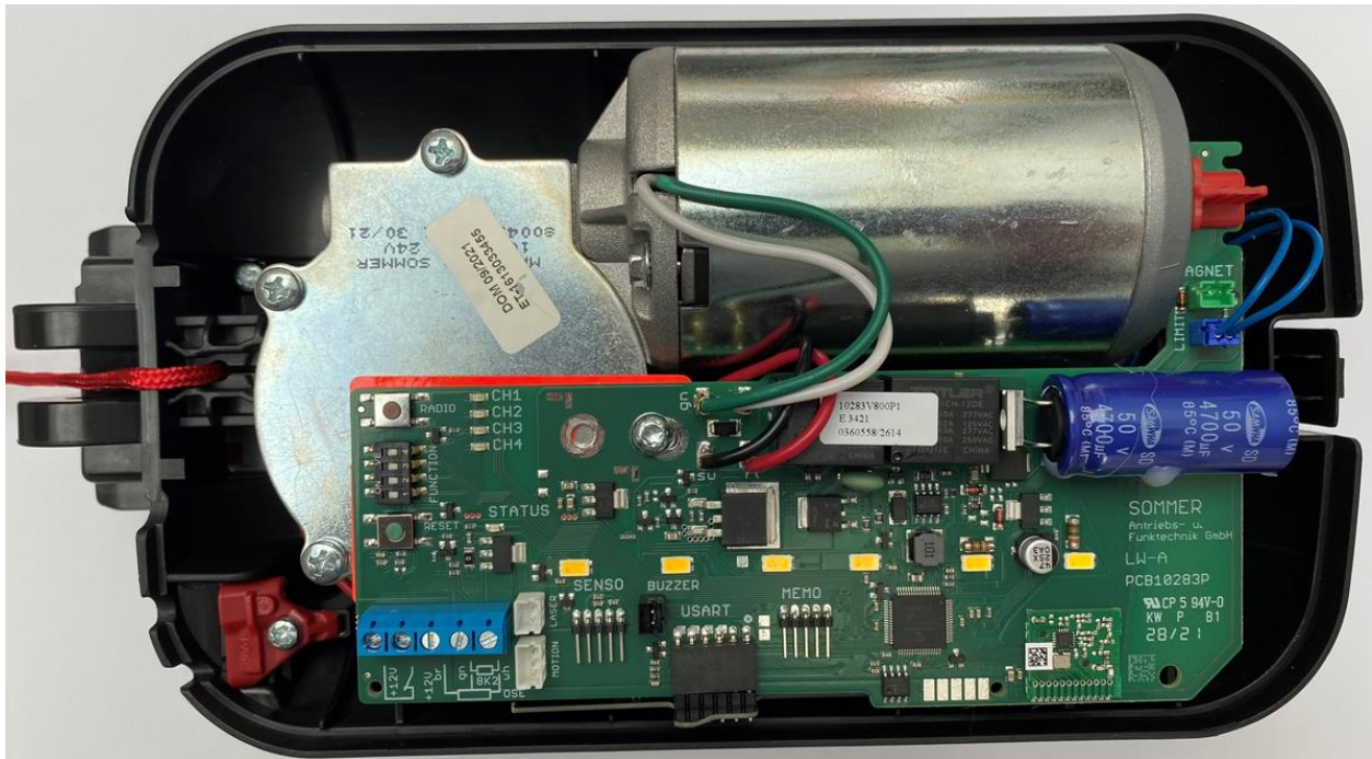
2080 PCB and Motor
