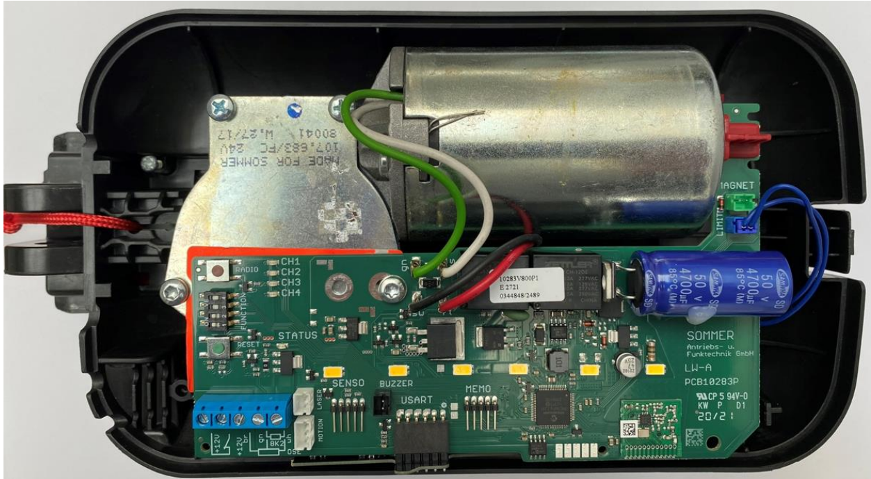
2060 PCB and Motor 1
