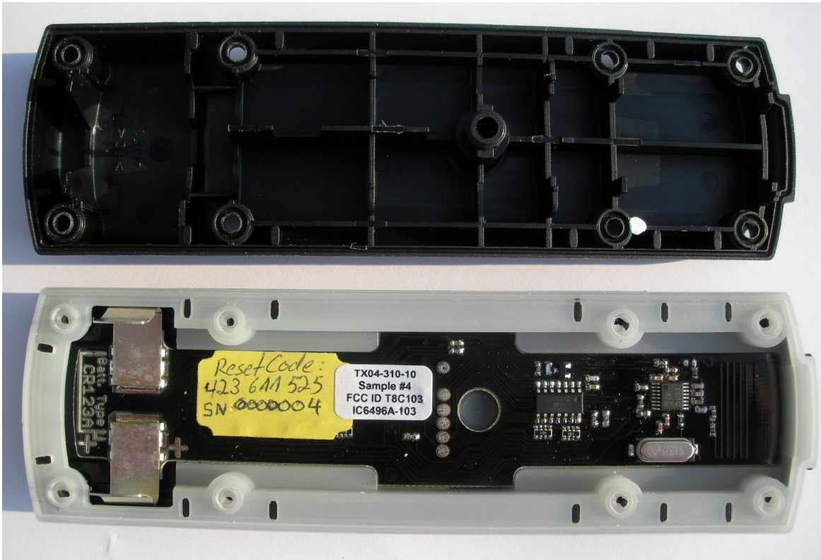
PCB inside the housing
