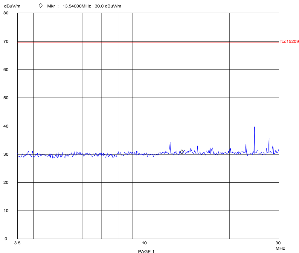
Plot 6.7.2: Magnetic Field emissions at 3m distance
