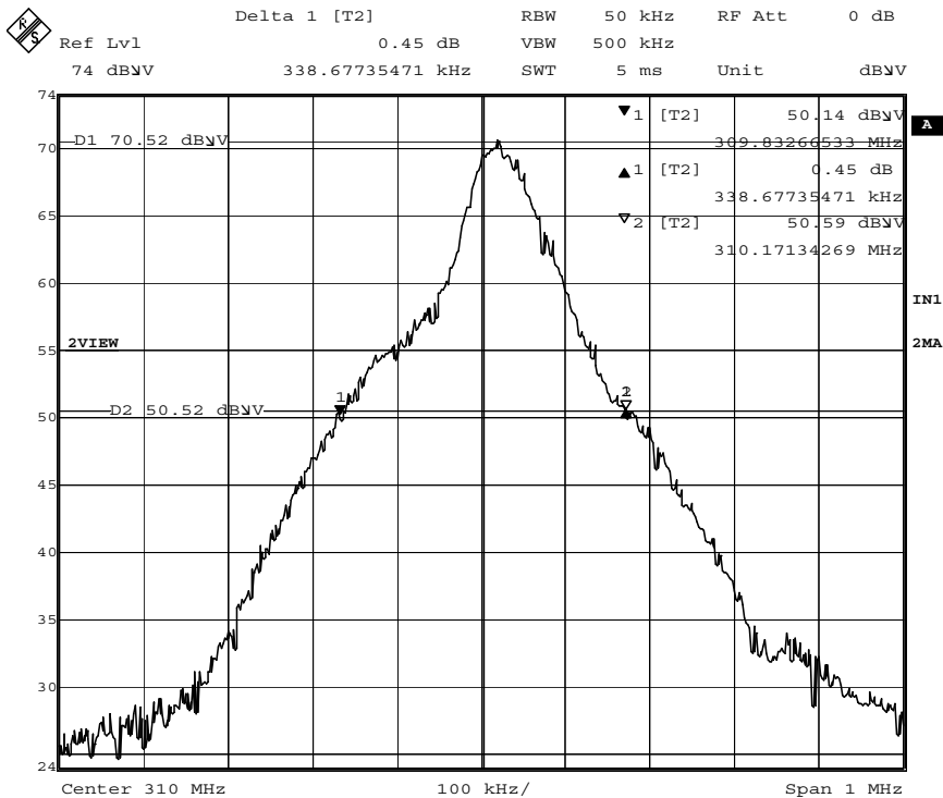
Plot 8.5-1: bandwidth plot – 20 dB bandwidth
