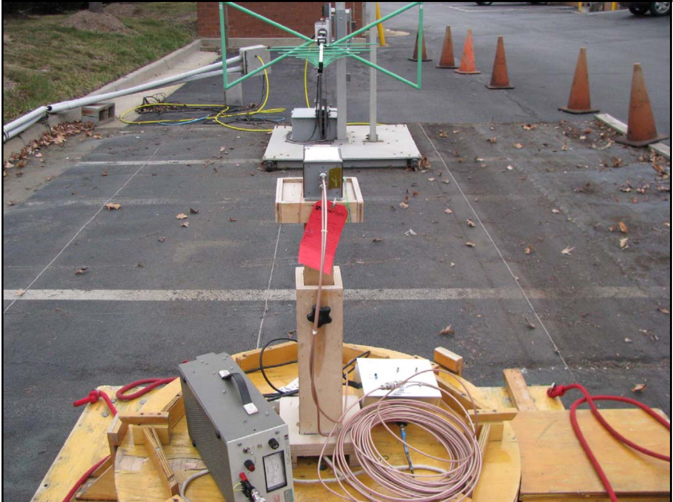
Photograph 1: Radiated TX Spurious Emissions – Front View
