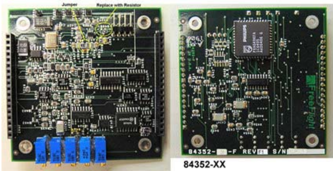
Fig 4 – 84352 MICROPROCESSOR BOARD
