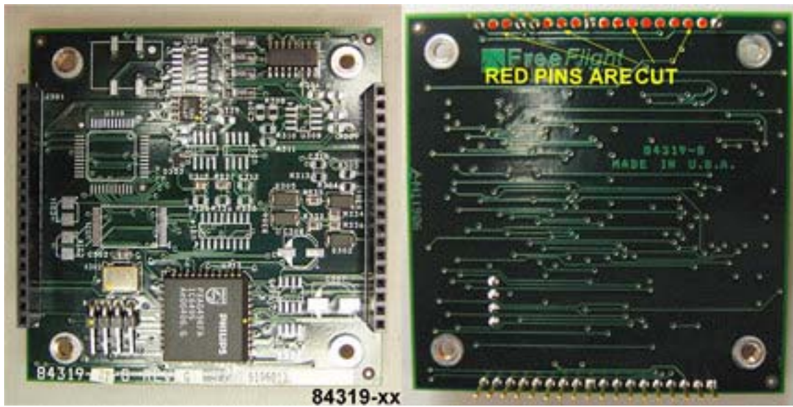
Fig 3 - 84319 I/O BOARD
