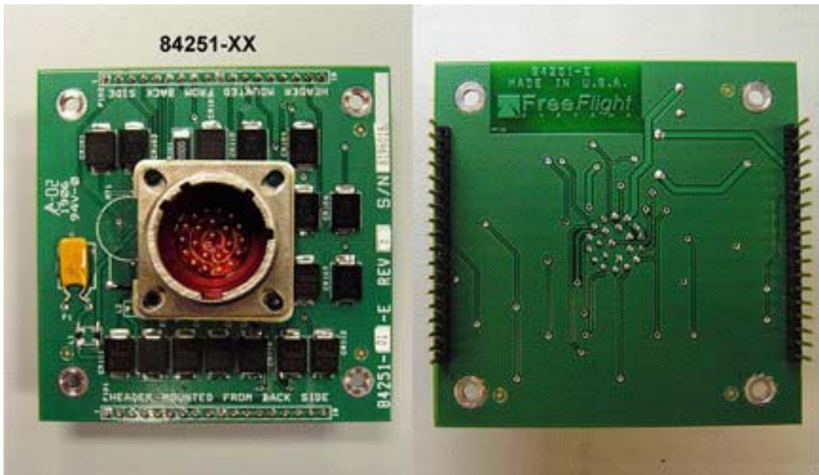
Fig 1 – 84251 FILTER BOARD
