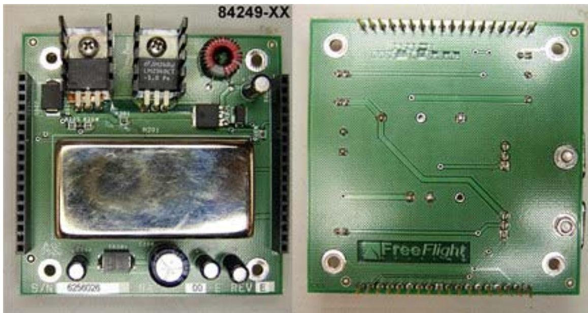
Fig 2 – 84249 POWER SUPPLY BOARD
