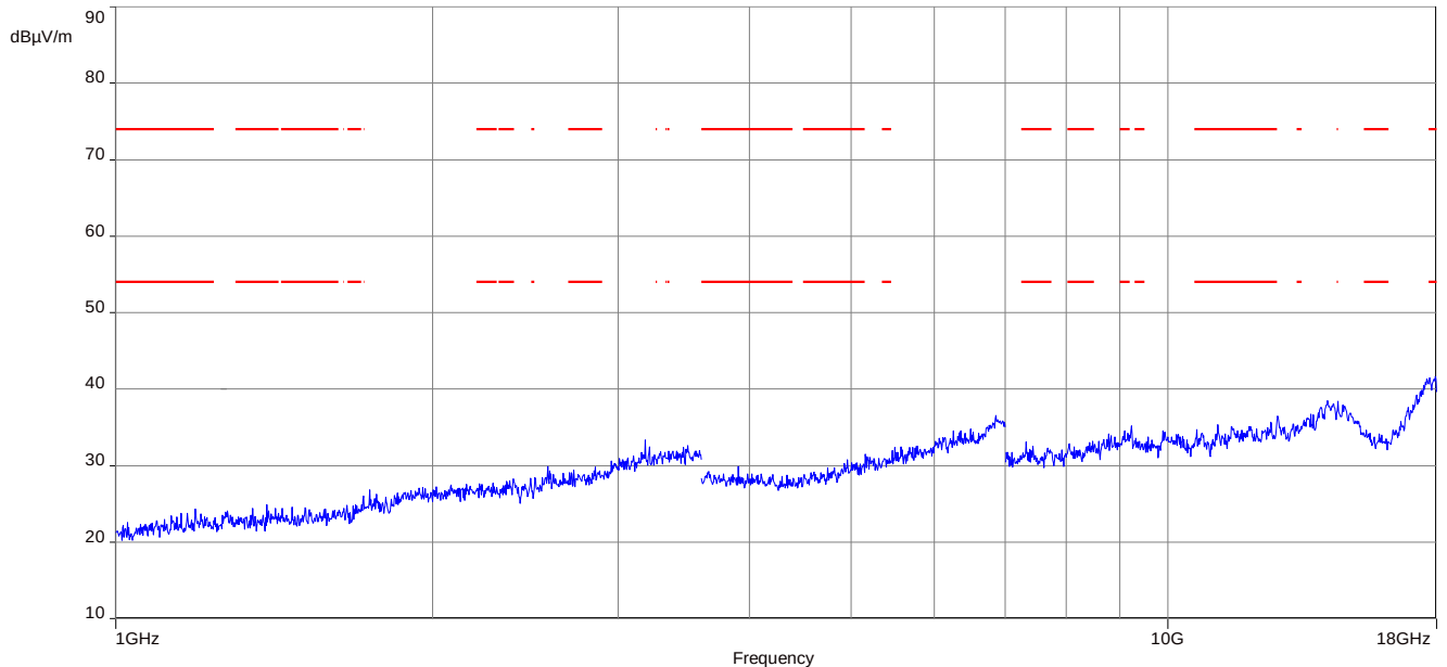
Plot 5: 1 GHz to 18 GHz, TX mode, 2480 MHz, vertical & horizontal polarization, O-QPSK
