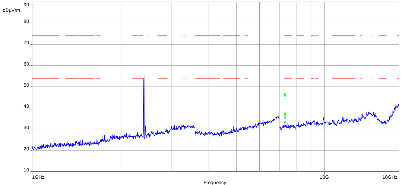
Plot 3: 1 GHz to 18 GHz, TX mode, 2440 MHz, vertical & horizontal polarization, O-QPSK
