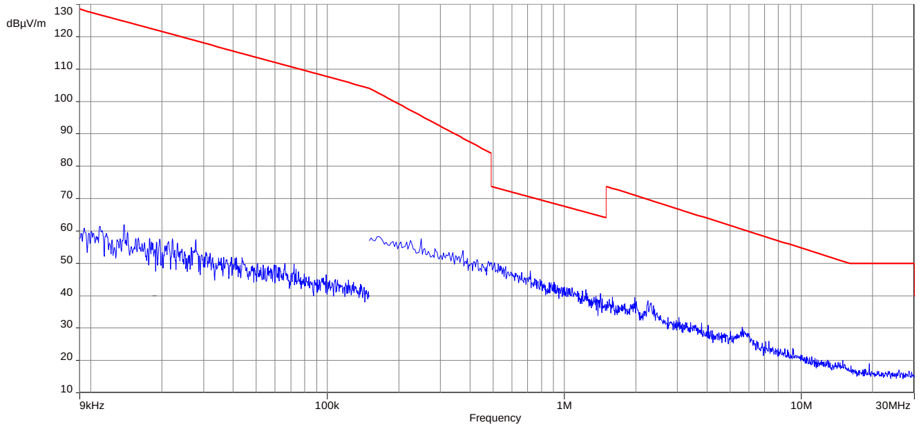
Plot 3: 9 kHz to 30 MHz, 2480 MHz, transmit mode, O-QPSK
