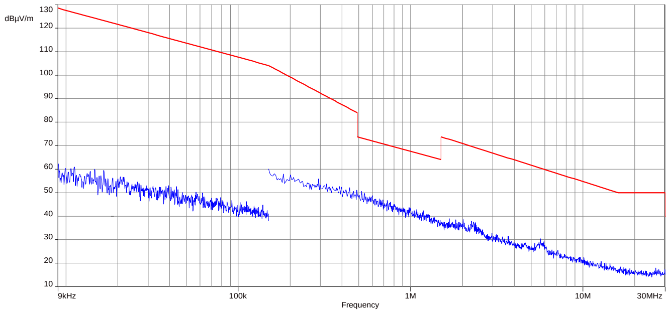
Plot 1: 9 kHz to 30 MHz, 2405 MHz, transmit mode, O-QPSK
