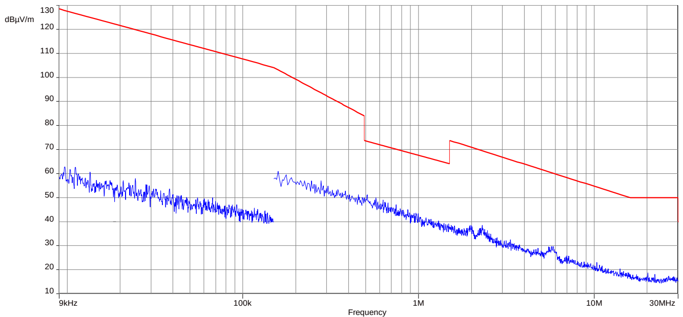
Plot 2: 9 kHz to 30 MHz, 2440 MHz, transmit mode, O-QPSK
