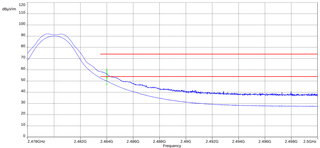
Plot 2: Upper restricted band, O-QPSK
