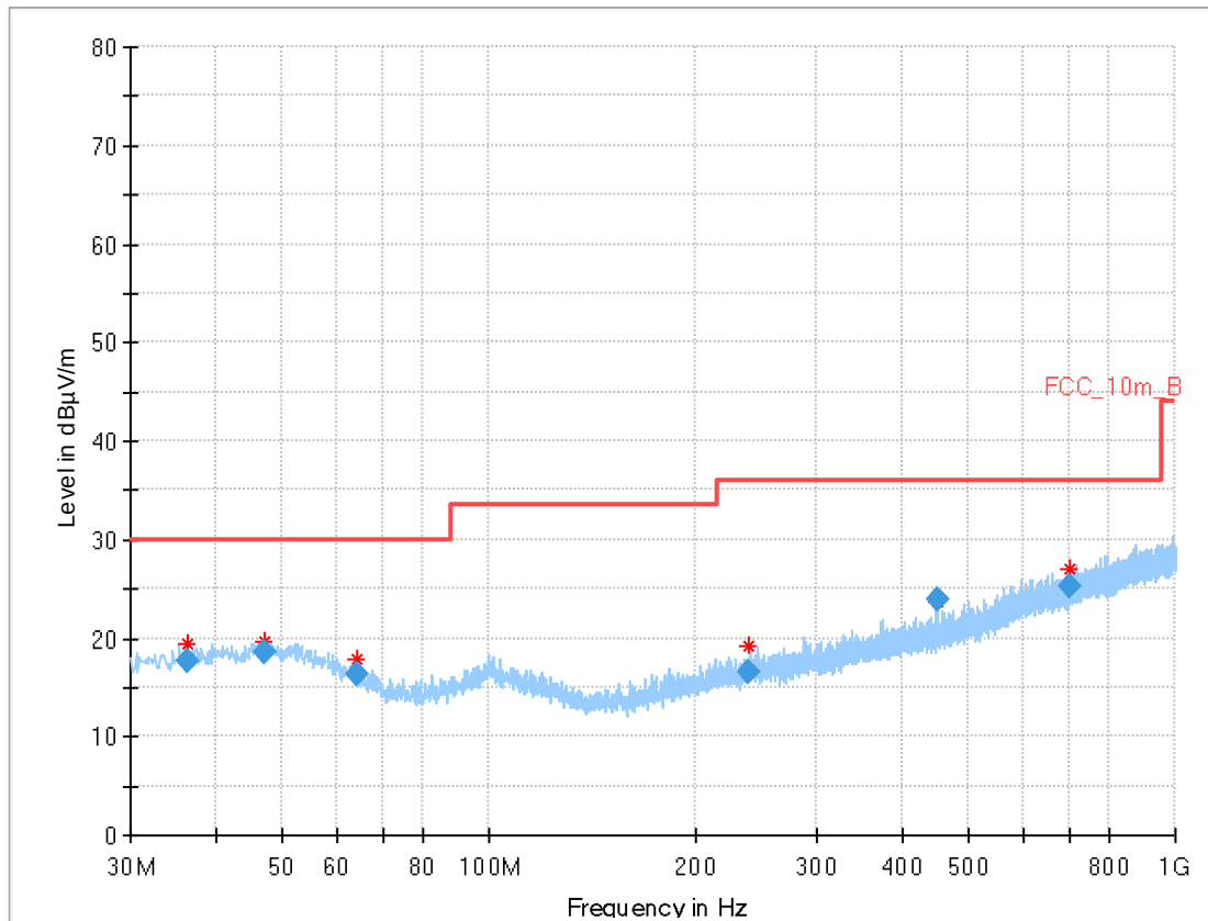
Plot 3: 30 MHz to 1 GHz, TX mode, 2480 MHz, vertical & horizontal polarization, O-QPSK
