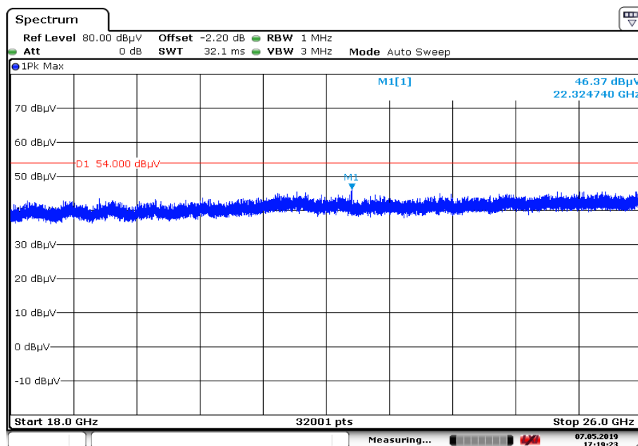
Plot 6: 18 GHz to 26 GHz, TX mode, 2480 MHz, vertical & horizontal polarization, O-QPSK
