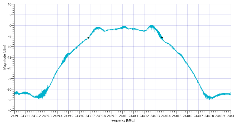
Plot_FCC Part 15.247 Maximum Peak Conducted Output Power DTS ~ BT LE 1 MspS DTS BW _06052019_162656.png
