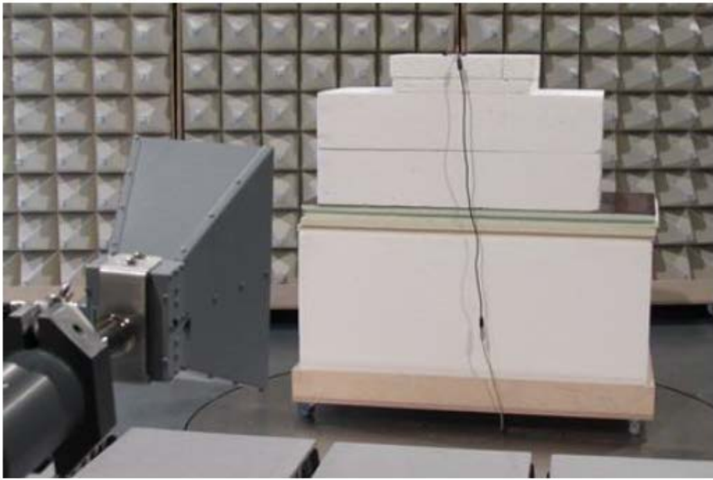
Radiated Setup C
