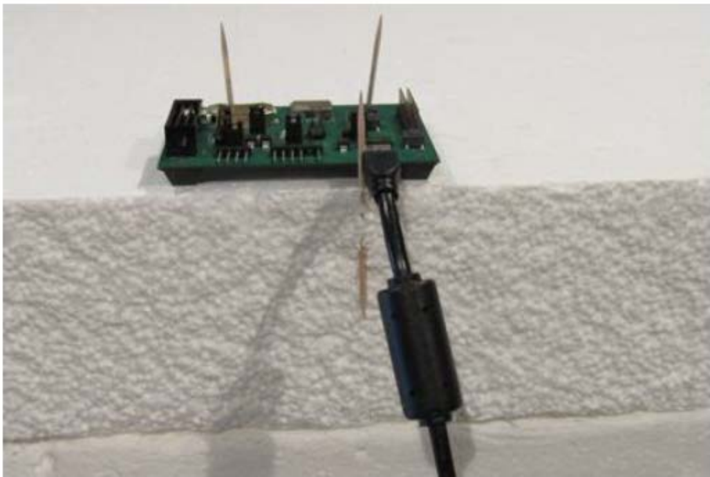
Radiated Setup Close Up View
