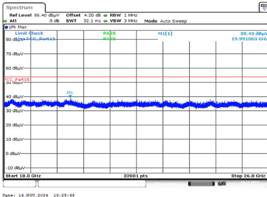
Plot 8: 18 GHz to 26 GHz, TX mode, vertical & horizontal polarization, valid for all channels
