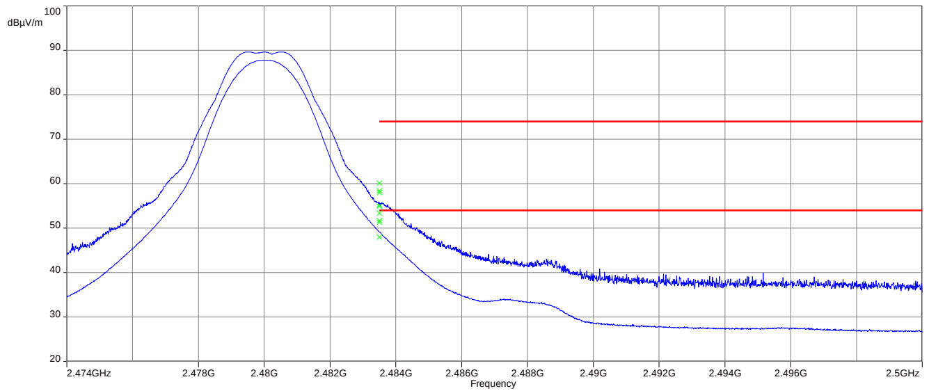
Plot 3: Upper restricted band, O-QPSK, 2480 MHz
