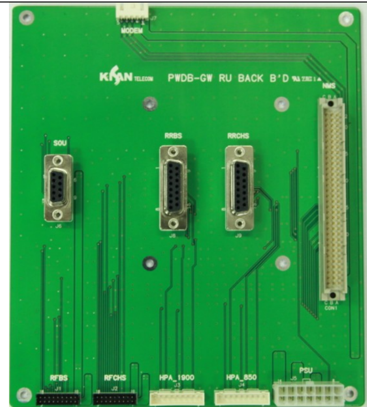
Interface B'd
