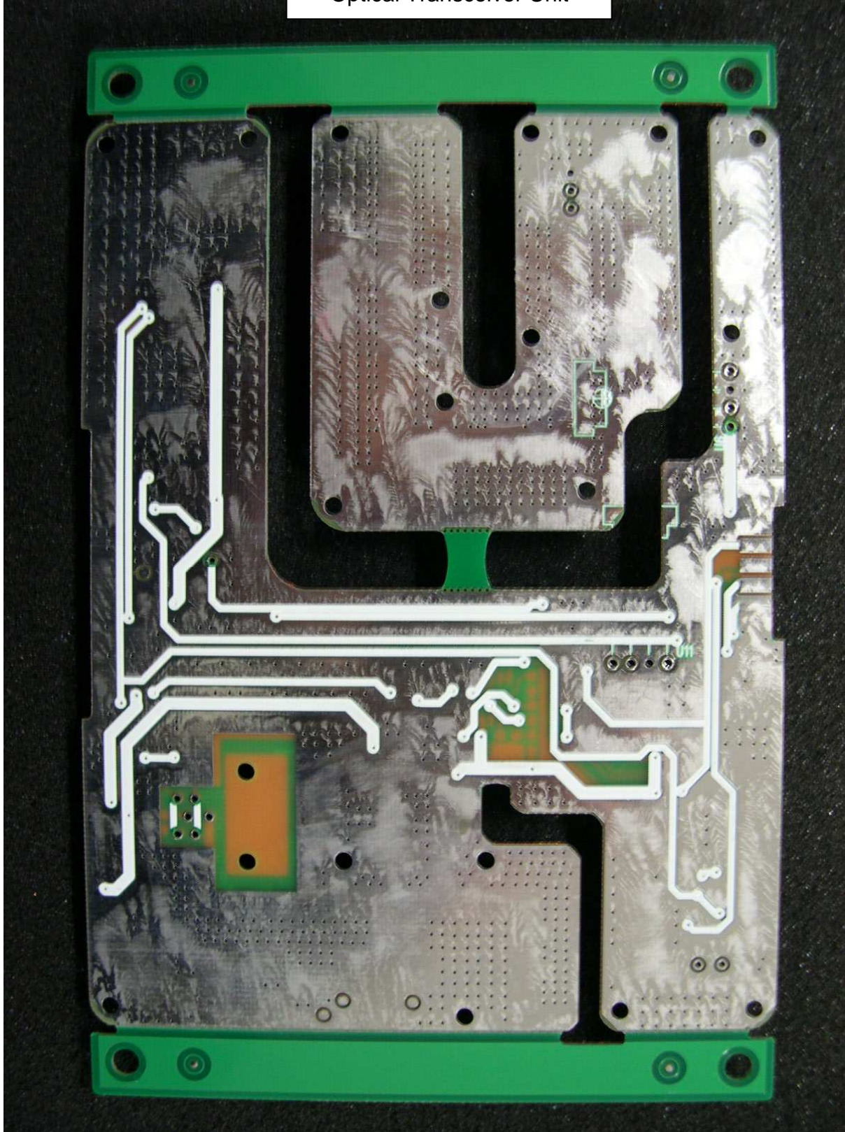
Optical Transceiver Unit
