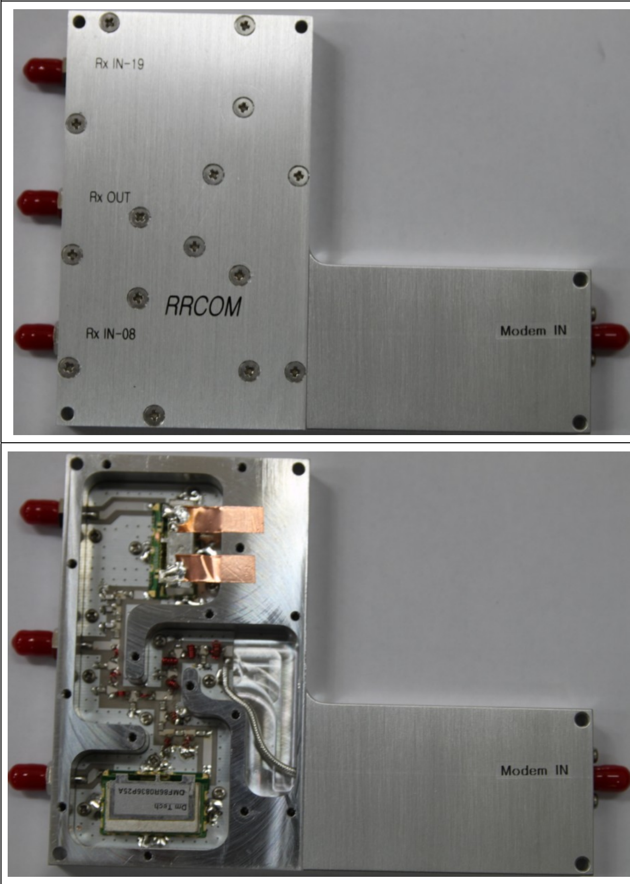
Combiner – RRCOM
