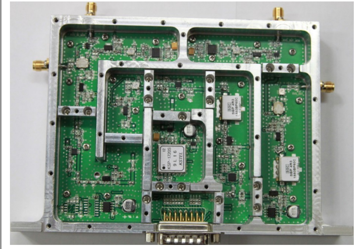
RRBS Pinout Table: 1:VCC 9:NC 2:GND 10:PLL CLK 3:NC 11:PLL DATA 4:ATT CLK 12:PLL EN1 5:ATT DATA 13:NC 6:OUT DET 14:PLL LD1 7:ATT EN1 15:NC 8:IN DET Labels on the board: RVS_IN_MON RVS_OUT_MON RVS_IN RVS_OUT KISAN TELECOM
