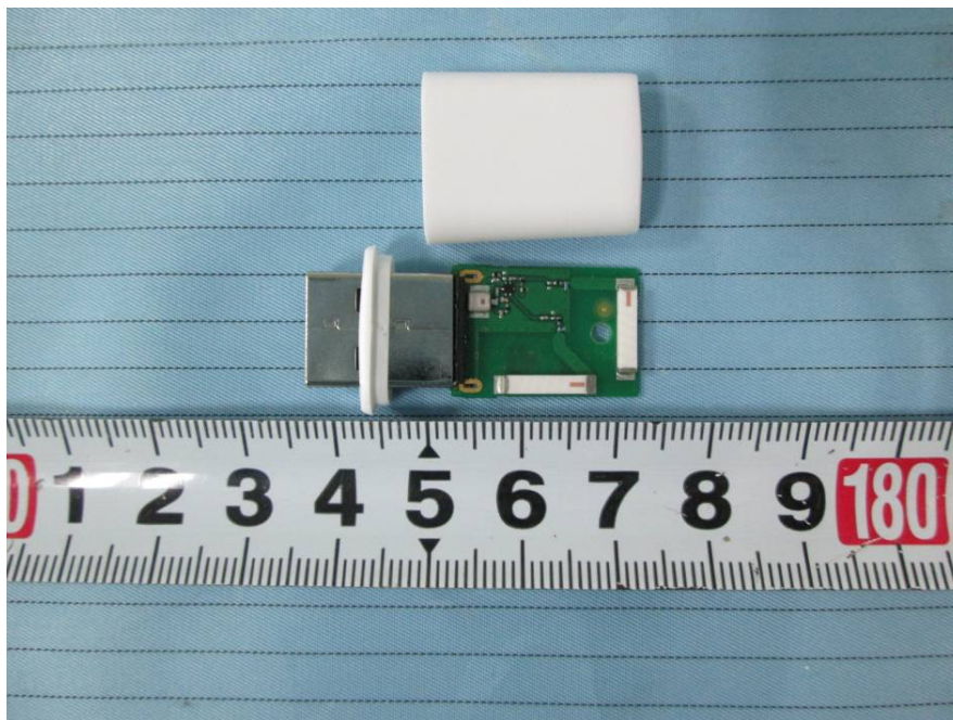
EUT – Cover off View (White Color)
