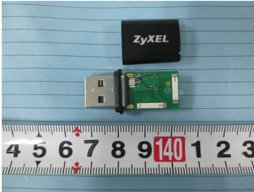
EUT – Cover off View (Black Color)
